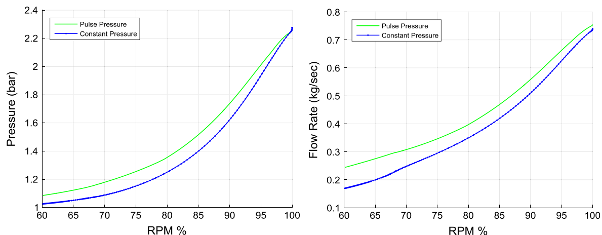
Fig. 5.6. Comparison between inlet receiver pressure (a) and air mass-flow rate (b) delivered by a pulse turbocharger and constant pressure turbocharger, with a 30 degree valve overlap engine.
