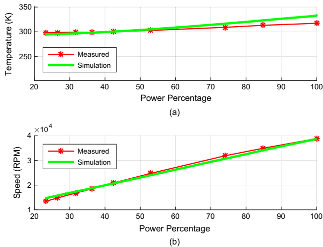
Fig. 3.2. Comparison between measured and simulated inlet receiver temperature (a), and turbocharger speed (b).
