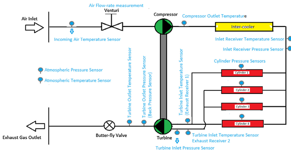
Fig. 2.3. Outline of test setup and sensor placement.
