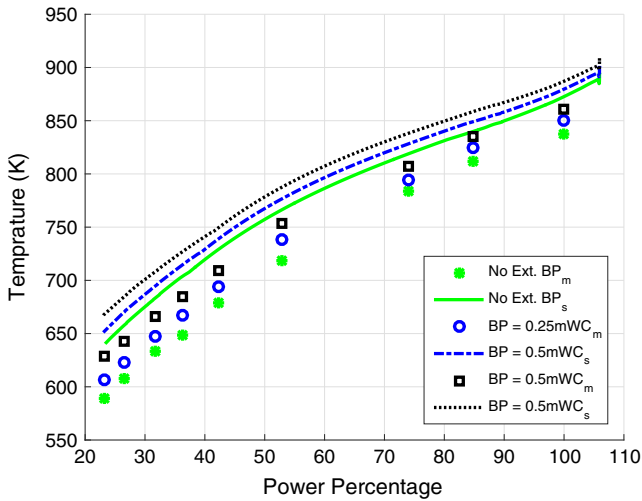
Fig. 4.5. Back pressure effect on turbine inlet temperature based on measurements (m) and simulations (s).
