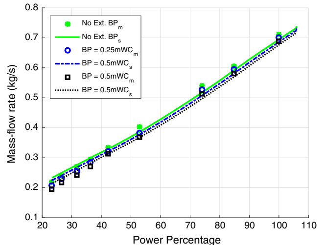
Fig. 4.3. Back pressure effect on air mass-flow rate based on measurements (m) and simulations (s).
