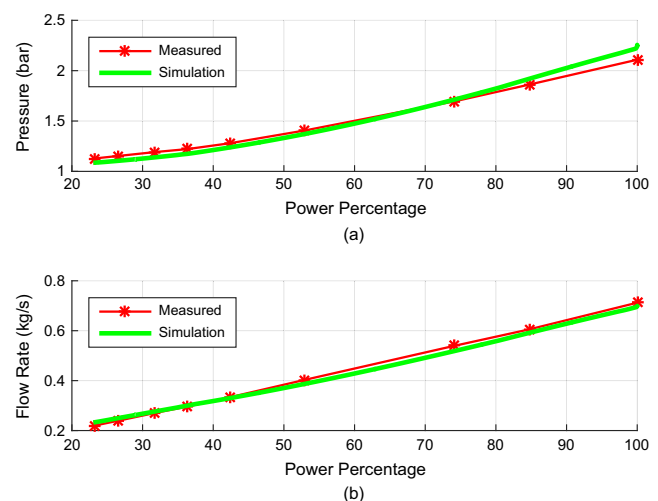
Fig. 3.1. Comparison between measured and simulated inlet receiver pressure (a), and air mass-flow rate (b).
