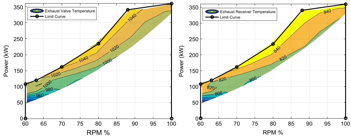
Fig. 5.3. Static engine map with lines of constant exhaust valve temperature (a) and constant exhaust receiver temperature (b) for a 100 degree valve overlap constant pressure turbocharged engine.
