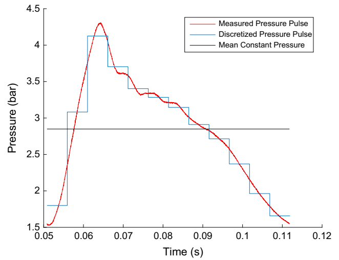
Fig. 2.8. Discretization of measured turbine inlet pressure pulse at 340 kW and 981 rpm.
