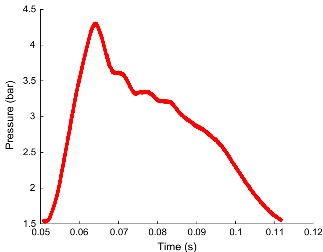
Fig. 2.5. Measured turbine inlet pressure pulse.
