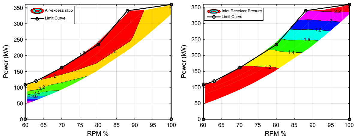
Fig. 5.2. Static engine map with lines of constant air-excess ratio (a), and lines of constant charge pressure (b) for a 100 degree valve overlap constant pressure turbocharged engine.
