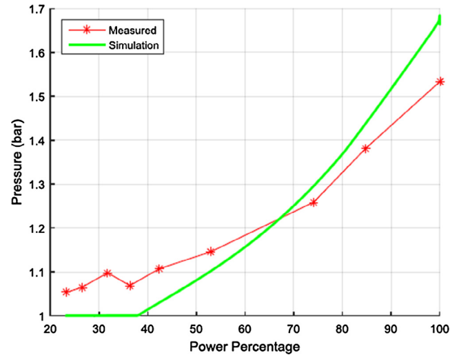
Fig. 3.4. Comparison between measured and simulated values of lowest turbine inlet pressure.
