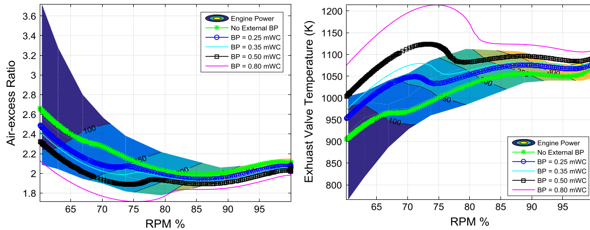
Fig. 5.5. Back pressure effect on air-excess ratio (a), and exhaust valve temperature (b) of a constant pressure turbocharged engine, with 30 degree valve overlap.
