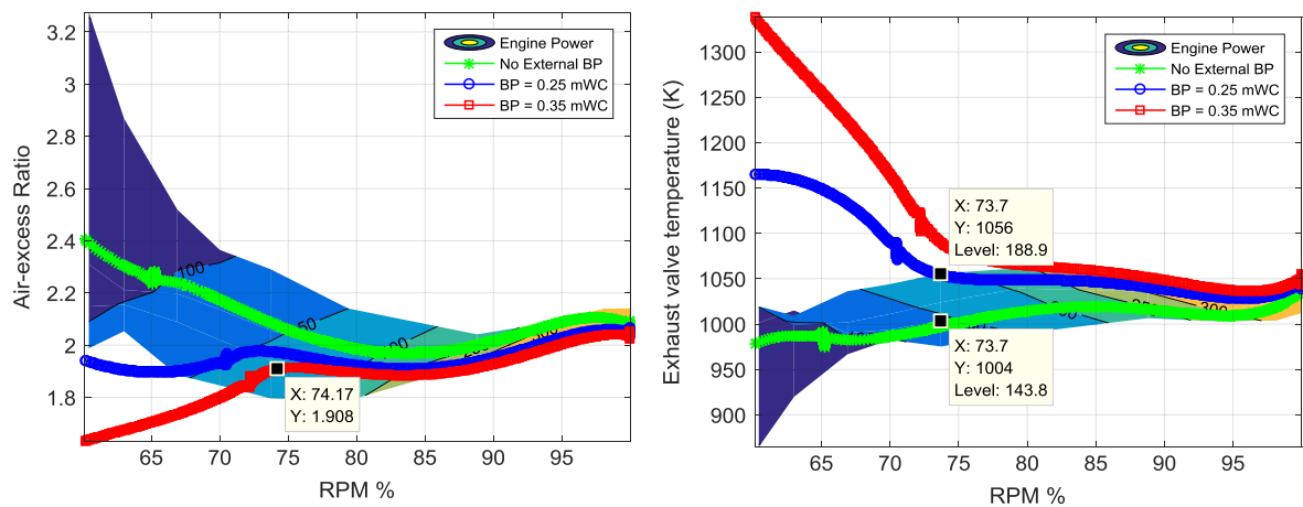
Fig. 5.4. Back pressure effect on air-excess ratio (a) and exhaust valve temperature (b) of a constant pressure turbocharged engine, with 100 degree valve overlap.
