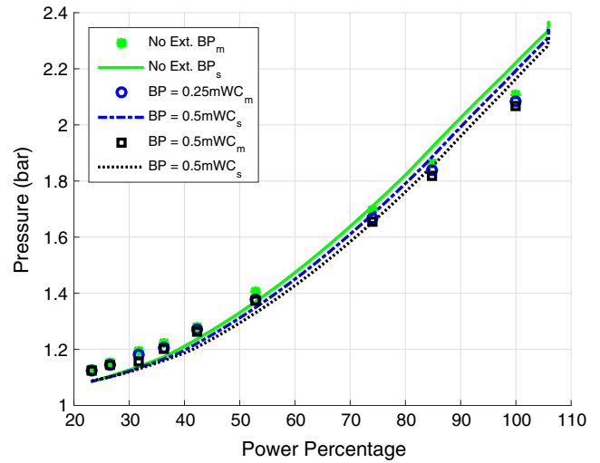
Fig. 4.2. Back pressure effect inlet receiver pressure based on measurements (m) and simulations (s).
