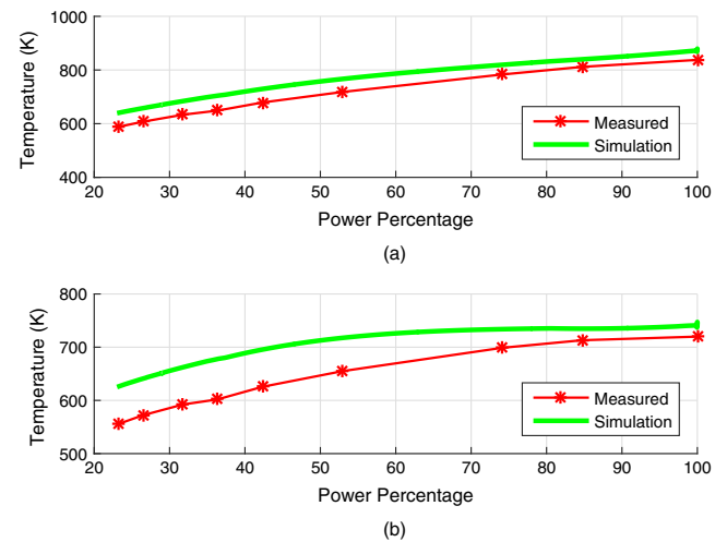
Fig. 3.5. Comparison between measured and simulated turbine inlet (a), and outlet temperatures (b).
