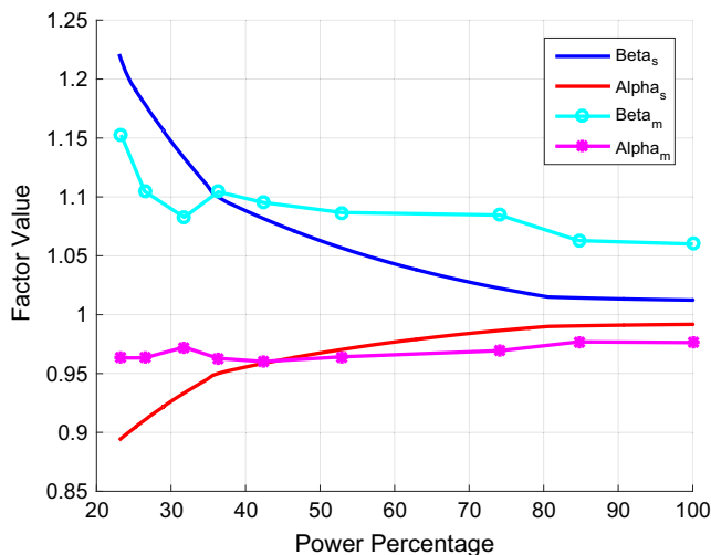
Fig. 3.3. Comparison between \alpha , \beta values obtained from simulation (s) and values calculated from measurements (m).
