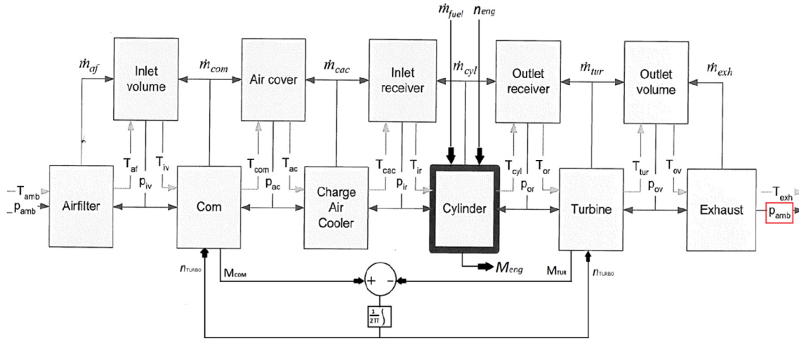
Fig. 2.4. Mean value engine model [41,42].
