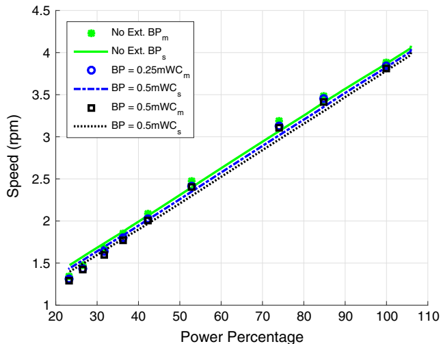
Fig. 4.1. Back pressure effect on turbocharger speed based on measurements (m) and simulations (s).
