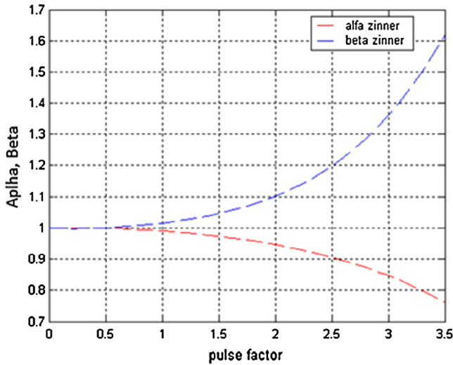
Fig. 2.7. Correction factors \alpha and \beta as a function of the pulse factor suggested by Zinner, according to Stapersma [44,51].
