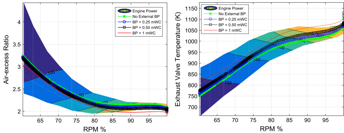
Fig. 5.7. Back pressure effect on air-excess ratio (a) and exhaust valve temperature (b) of a constant pressure turbocharged engine, with 30 degree valve overlap.
