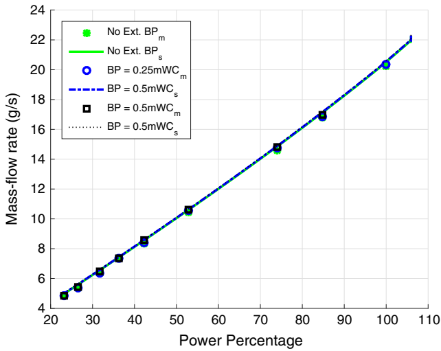
Fig. 4.4. Back pressure effect on fuel consumption based on measurements (m) and simulations (s).
