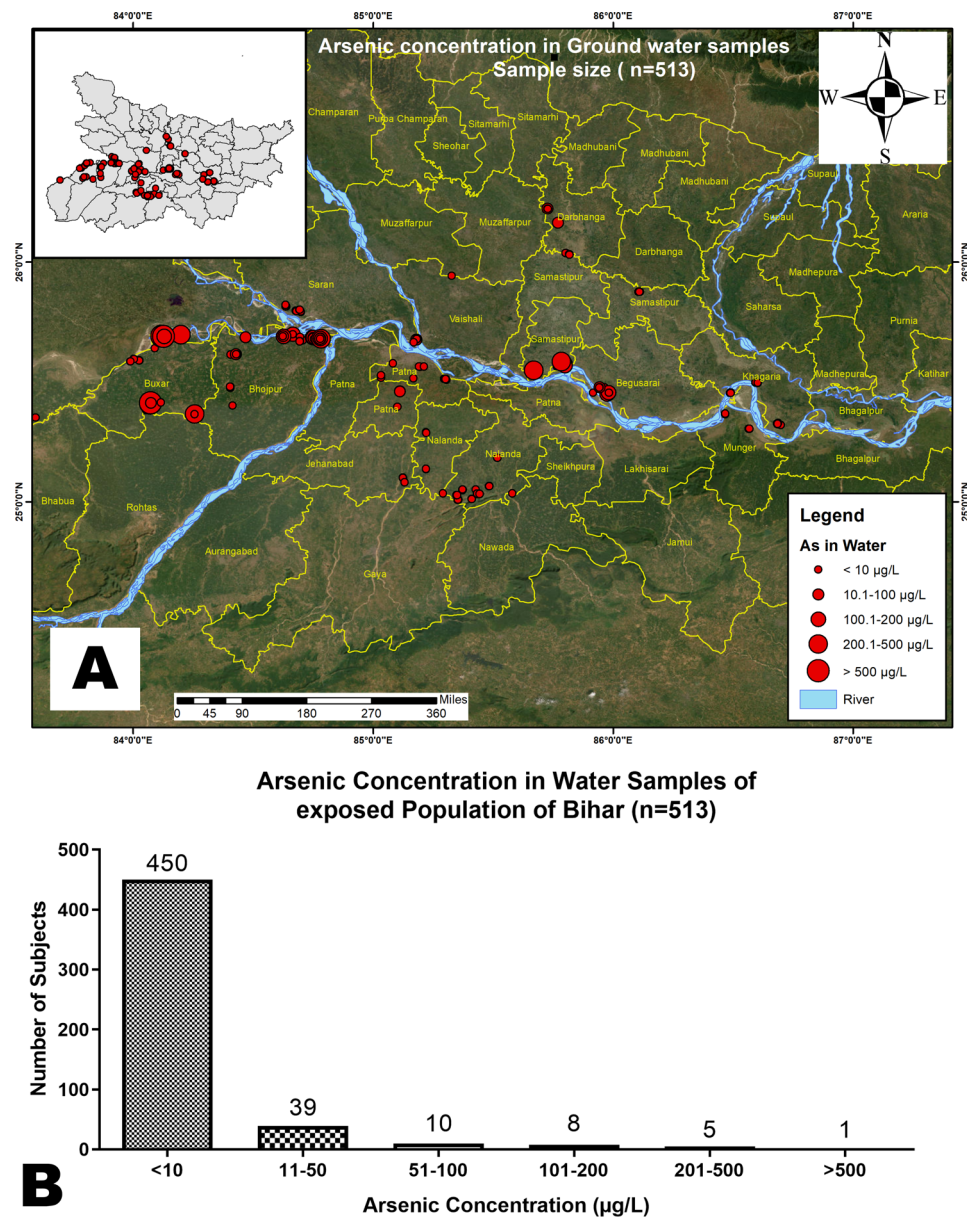
Fig. 2 A Showing geospatial maps of studied arsenic 11 hotspot districts with groundwater poisoning. B Showing the graph with the levels of arsenic concentration in the drinking water samples of exposed districts
