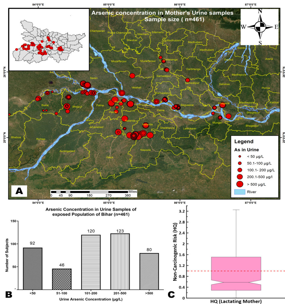
Fig. 5 A Showing geospatial maps of studied arsenic 11 hotspot districts with arsenic poisoning in the mother's urine samples of the subjects. B Showing the graph with the levels of arsenic concentration in the mother's urine samples of subjects of exposed districts. C Human health risk assessment (HQ) - non-carcinogenic risk in lactating mothers
