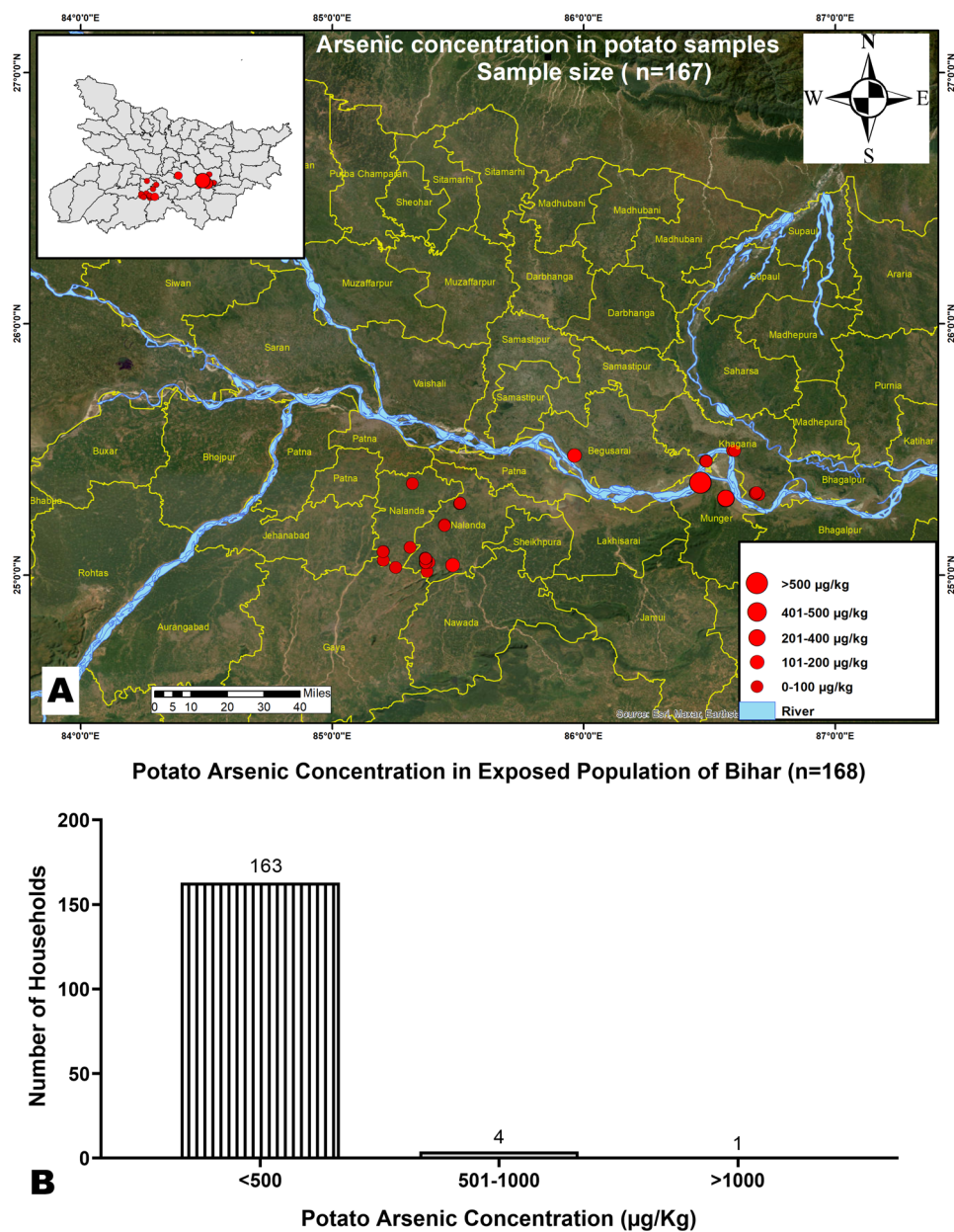
Fig. 9 A Showing geospatial map of studied arsenic 10 hotspot districts with arsenic poisoning in the potato samples of the households. B Showing the graph with the levels of arsenic concentration in the potato samples of households of exposed districts
