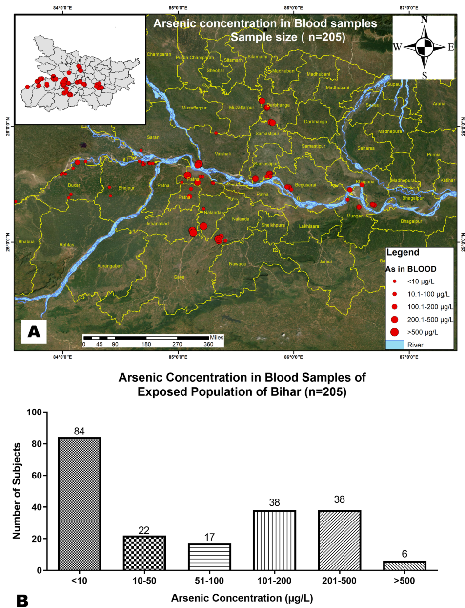
Fig. 3 A Showing geospatial maps of studied arsenic 11 hotspot districts with arsenic poisoning in the blood samples. B Showing the graph with the levels of arsenic concentration in the blood samples of subjects of exposed districts
