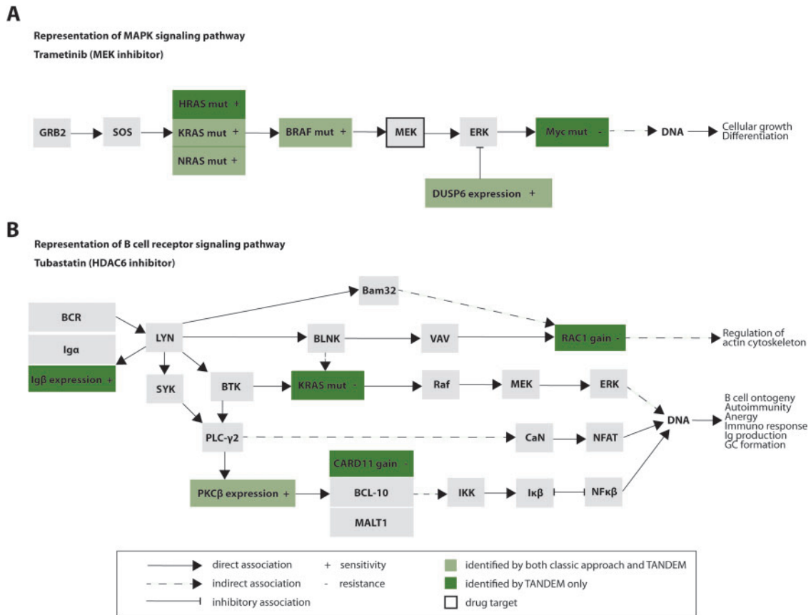
Fig. 4. Features selected by TANDEM in the context of two pathways. Representation of (A) the MAPK signaling pathway and (B) the B cell receptor signaling pathway from KEGG. Indicated in color are the genes associated with response to (A) Trametinib or (B) Tubastatin by TANDEM (dark green) or by both approaches (light green)
