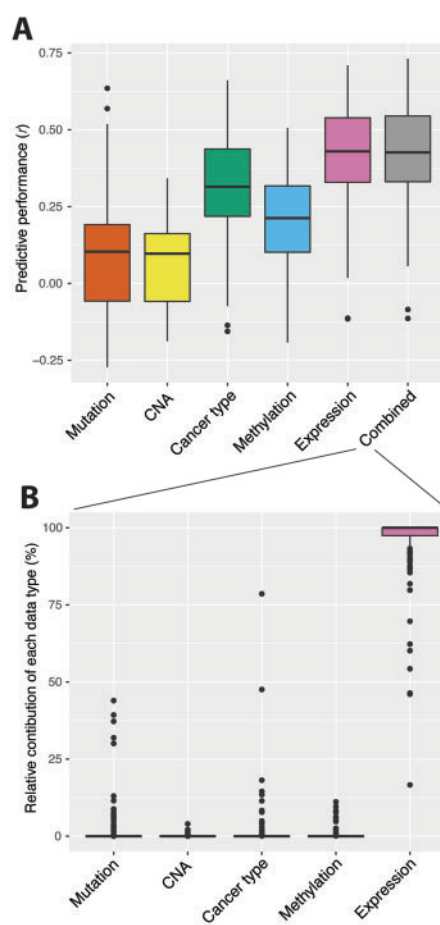
Fig. 2. Predictive performance of individual molecular data types. (A) Predictive performance (Pearson correlation between measured IC50s and predictions from the classic approach) across 265 drugs using individual data types (mutation, CNA, tissue of origin, methylation, gene expression) or a combination of all data types (combined) with the classic approach. (B) Relative contribution of each data type in the combined models, across all drugs for which we achieved a predictive performance r > 0.4
