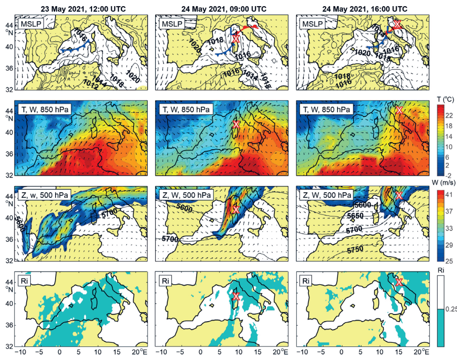
Figure 4. Synoptic conditions during the May 2021 meteotsunami event. (First row) mean sea-level pressure and temperature fronts; (second row) temperature (shaded) and wind at 850 hPa; (third row) geopotential height and wind at 500 hPa (wind speeds above 25 m/s are shown in colour); (fourth row) unstable atmospheric layers (coloured areas denote Ri < 0.25 ); (first column) 23 rd of May 2021, 12:00 UTC; (second column) 24 th of May 2021, 09:00 UTC; (third column) 24 th of May 2021, 16:00 UTC. The crosses mark the locations where meteotsunamis occurred and are indicated at the times closest to meteotsunami occurrence.
