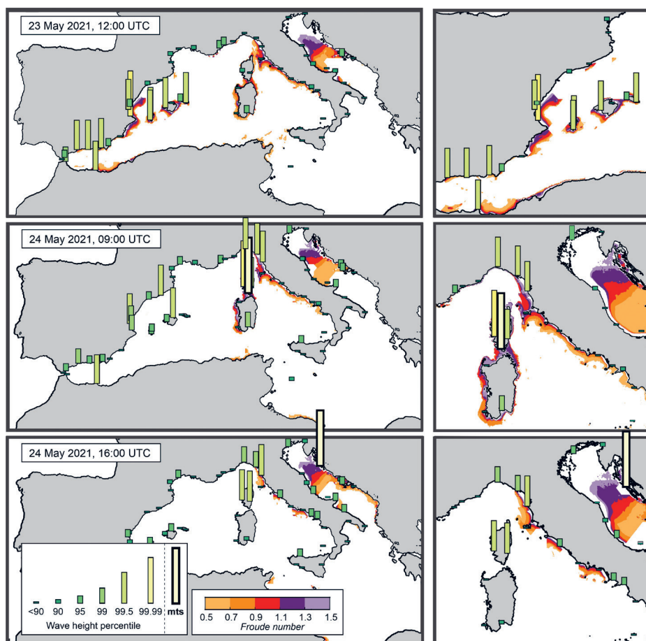
Figure 6. Froude number at the western Mediterranean and the Adriatic Seas on: (top row) 23 rd of May 2021, 12:00 UTC; (middle row) 24 th of May 2021, 09:00 UTC; (bottom row) 24 th of May 2021, 16:00 UTC. The plots on the right are zoom-ins of plots on the left. The maximum wave heights in one hour centred around the given times are shown in relation to the heights of the typical oscillations at each station. The meteotsunami heights are also shown, with an assumption that their heights are near the 100 th percentile of the respective background heights.
