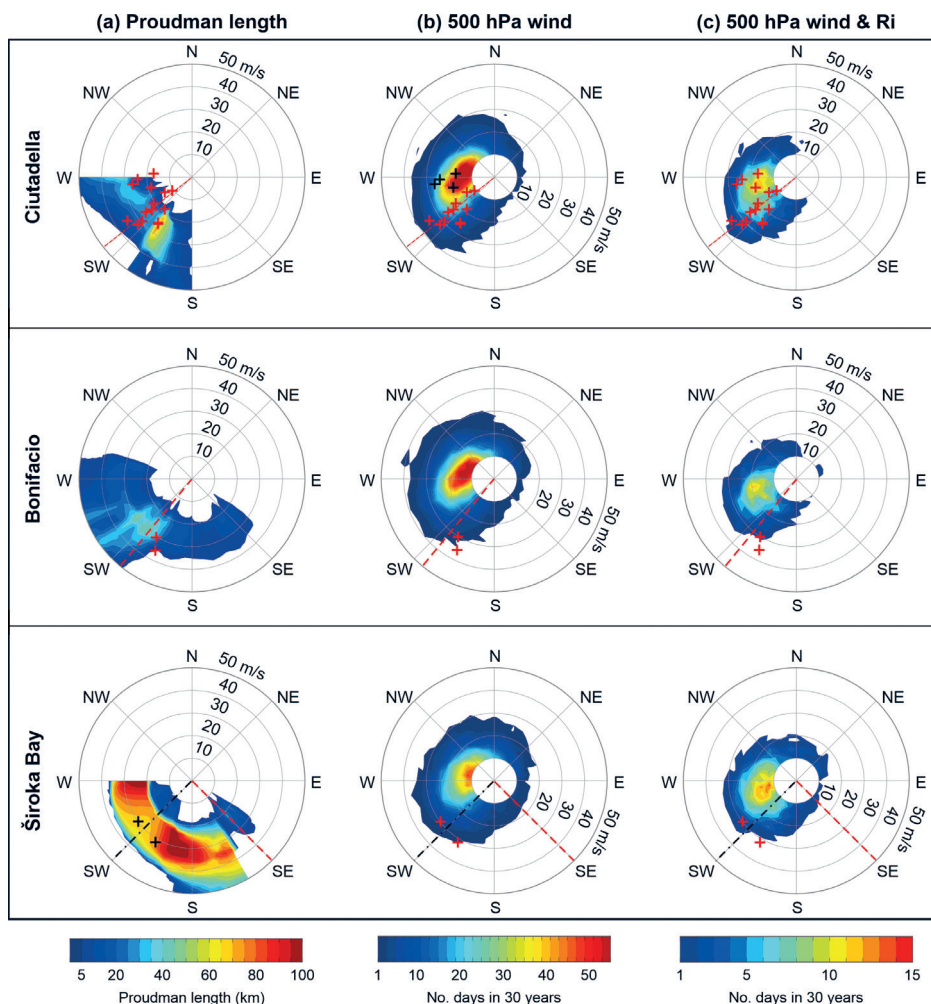
Figure 13. (a) Proudman length; (b) climatology of the 500-hPa wind; and (c) climatology of the 500-hPa wind on days when atmospheric layers between 600 and 400 hPa are unstable; for (first row) Ciutadella; (second row) Bonifacio and (third row) Široka Bay. Red dashed lines denote orientation of bay mouths; and black dot-dashed line orientation of the narrow strait between the islands of Ist and Molat (as indicated in Fig. 1).
