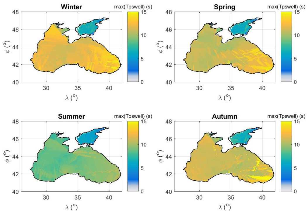
Figure 10. Spatial variation of the maximum peak period of swell waves per season based on hindcast results from 1979-2009.
