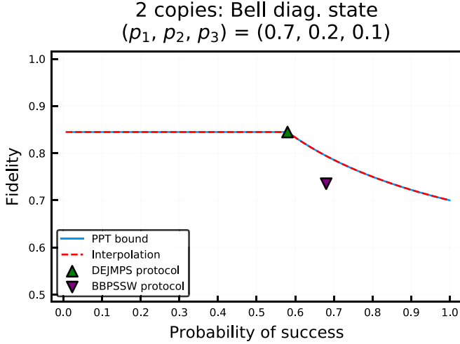
FIG. 3. Distilling the Bell diagonal states of rank-three \tau_{ab}^{\otimes 2} with D = 2 and p_1 = 0.7, p_2 = 0.2, p_3 = 0.1 in Eq. (37) to a two-qubit state. The fidelity of each input copy is F_{\text{in}} = 0.7 and we observe that deterministic distillation (with p_{\text{succ}} = 1 ) is not possible for two copies of this state. We see that DEJMPS is optimal for a mixture of three Bell states. Moreover, extrapolating from DEJMPS to higher probability of success as described in Appendix B 2, we see that the extrapolation curve overlaps with the PPT bound for all values of the probability of success. This means that this extrapolation also results in optimal schemes achieving the highest possible output fidelity for the specific fixed probability of success. The 1-BSE bound is not included because it overlaps with the PPT bound.
