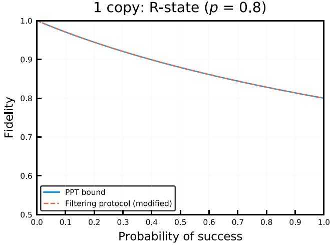
FIG. 6. Filtering R state \tau_{AB} with D = 2 and p = 0.8 in Eq. (42) to a two-qubit state. The fidelity of the input copy is F_{\text{in}} = 0.8 and in accordance with [47] we observe that deterministic filtering (with p_{\text{succ}} = 1 ) is not possible for this state. We see that the filtering scheme perfectly overlaps with the PPT bound, which proves its optimality for this state. The 1-BSE bound is not included because it overlaps with the PPT bound.
