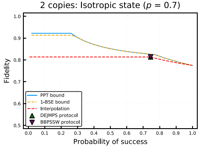
FIG. 1. Distilling the isotropic states \tau_{ab}^{\otimes 2} with D = 2 and p = 0.7 in Eq. (32) to a two-qubit state. The fidelity of each input copy is F_{\text{in}} = 0.775 and we observe that deterministic distillation (with p_{\text{succ}} = 1 ) is not possible for two copies of the isotropic state. We also find that the method of 1-BSE provides tighter bounds than the PPT method alone.
