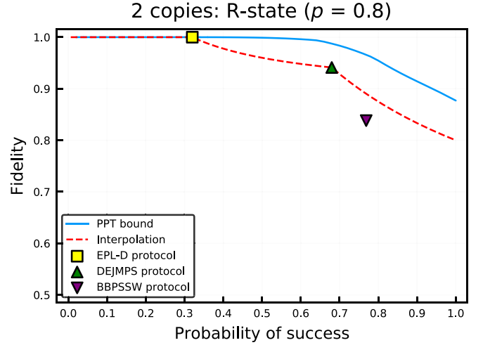
FIG. 8. Distilling the R states \tau_{ab}^{\otimes 2} with D = 2 and p = 0.8 in Eq. (42) to a two-qubit state. The fidelity of the input copy is F_{\text{in}} = 0.8 and we observe that while the extrapolation from DEJMPS does not allow for deterministic distillation (with p_{\text{succ}} = 1 ) in this case, the PPT bound still allows for this possibility. We also see that EPL-D allows for achieving unit fidelity. The 1-BSE bound is not included because it overlaps with the PPT bound.
