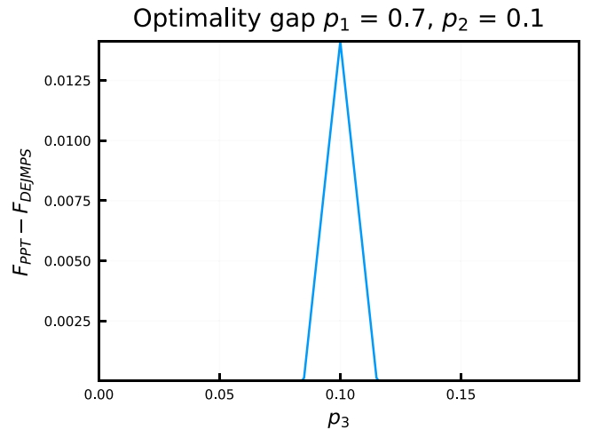
FIG. 5. Distilling the Bell diagonal states of rank-four \tau_{ab}^{\otimes 2} with D = 2 and p_1 = 0.7, p_2 = 0.1 in Eq. (37) to a two-qubit state. The fidelity of each input copy is F_{\text{in}} = 0.7 . The plot shows the difference between the PPT bound and the fidelity achievable through DEJMPS as a function of p_3 for the probability of success of DEJMPS. We see that DEJMPS achieves the highest possible output fidelity for this protocol's probability of success for a mixture of four Bell states which are far enough from the isotropic state (the middle of the peak). Clearly the states considered on this plot for which p_3 \neq 0.1 do not satisfy the condition p_1 > p_2 \geq p_3 \geq 1 - p_1 - p_2 - p_3 ; therefore when applying the DEJMPS protocol to such a state we first permute the Bell coefficients to this order. The 1-BSE bound is not included because it overlaps with the PPT bound.
