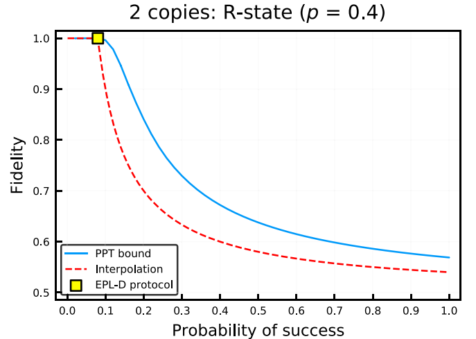
FIG. 9. Distilling the R states \tau_{ab}^{\otimes 2} with D = 2 and p = 0.4 in Eq. (42) to a two-qubit state. The fidelity of the input copy is F_{\text{in}} = 0.4 and we observe that deterministic distillation (with p_{\text{succ}} = 1 ) which achieves output fidelity larger than half is easily achievable for two copies of this state. We also see that EPL-D allows for achieving unit fidelity even if p \leq 0.5 . The 1-BSE bound is not included because it overlaps with the PPT bound.
