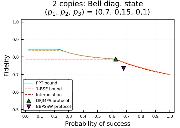
FIG. 4. Distilling the Bell diagonal states of rank-four \tau_{ab}^{\otimes 2} with D = 2 and p_1 = 0.7, p_2 = 0.15, p_3 = 0.1 in Eq. (37) to a two-qubit state. The fidelity of each input copy is F_{\text{in}} = 0.7 and we observe that deterministic distillation (with p_{\text{succ}} = 1 ) is not possible for two copies of this state. We also find that the 1-BSE bound is tighter than the PPT bound for smaller values of the probability of success. Finally, we observe that DEJMPS achieves the highest possible output fidelity for this protocol's probability of success for a mixture of four Bell states which are far enough from the isotropic state.
