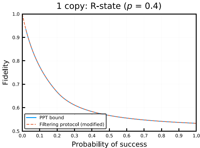
FIG. 7. Filtering R state \tau_{AB} with D = 2 and p = 0.4 in Eq. (42) to a two-qubit state. The fidelity of the input copy is F_{\text{in}} = 0.4 . As first shown in Ref. [47], we observe that for the smaller values of p deterministic filtering of R states is possible and can be achieved with our scheme. We also see that the filtering scheme perfectly overlaps with the PPT bound, which proves its optimality for this state. The 1-BSE bound is not included because it overlaps with the PPT bound.
