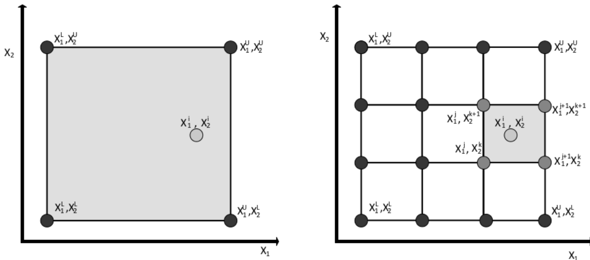
(a) MPI approach: the trajectory is computed by using the four extremal trajectories, which represent the database. (b) AMPI approach: given the larger database, four neighbor trajectories around the off-nominal conditions are selected, and used to compute the trajectory.
