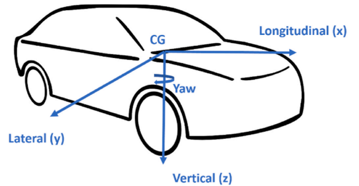
Fig. 5. The coordinate system of a vehicle. CG is the centre of gravity.
