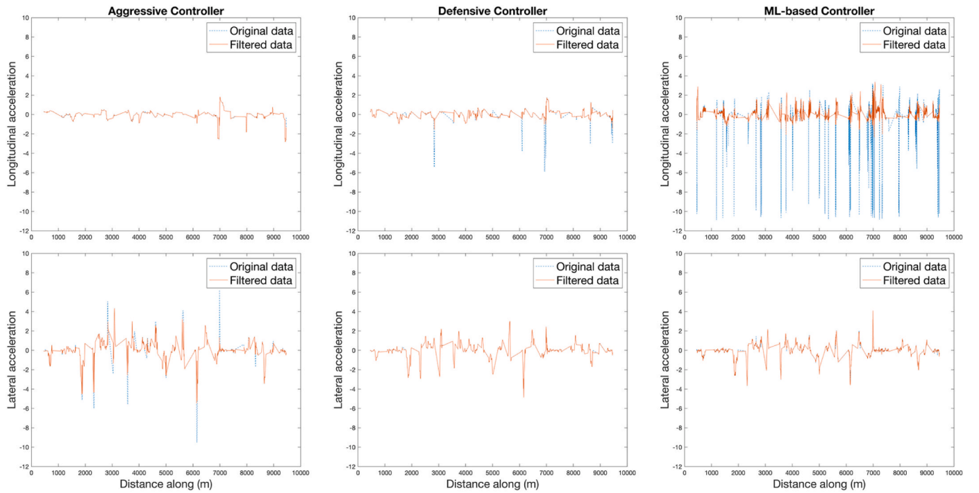
Fig. 4. The original and filtered longitudinal and lateral acceleration values of the three controllers.
