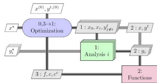
Fig. 7 XDSM for an individual discipline feasible (IDF) architecture [19]
