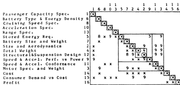
Fig. 6 Design structure matrix (DSM) [29]
