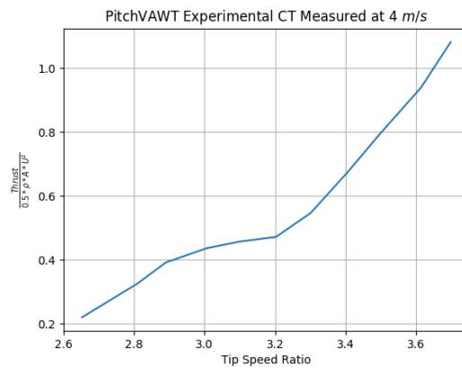
Figure 12. Measured CT vs Tip Speed Ratio for PitchVAWT with Zero degree fixed pitch
