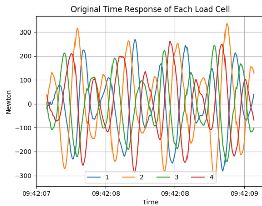
Figure 5. Unfiltered time response of each load cell at TSR 3.25
