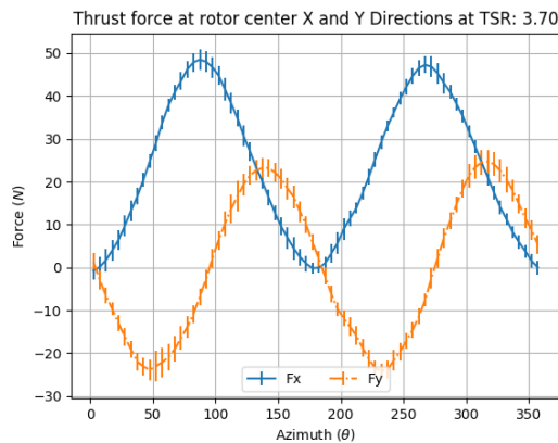
Figure 11. Thrust force at a wind speed of 4.01 \frac{m}{s} and a TSR of 3.7 over 22 rotations with standard deviation. \overline{\sigma_{F_x}} = 1.9N ; \overline{\sigma_{F_y}} = 2.3N
