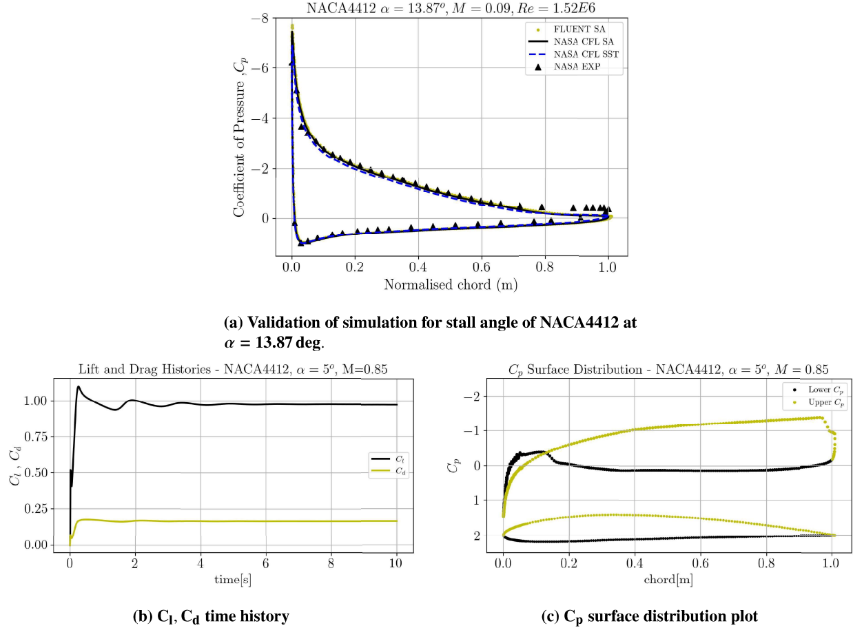
Fig. 3 CFD Steady and uRANS simulation of a NACA4412 airfoil (static) at \alpha = 5 deg, M = 0.85 .
