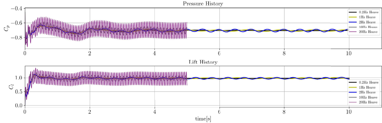
Fig. 4 CFD uRANS simulation of a NACA4412 airfoil (Heave dynamics) at H = \pm 0.1m , \alpha_0 = 5 deg, M = 0.85 .
