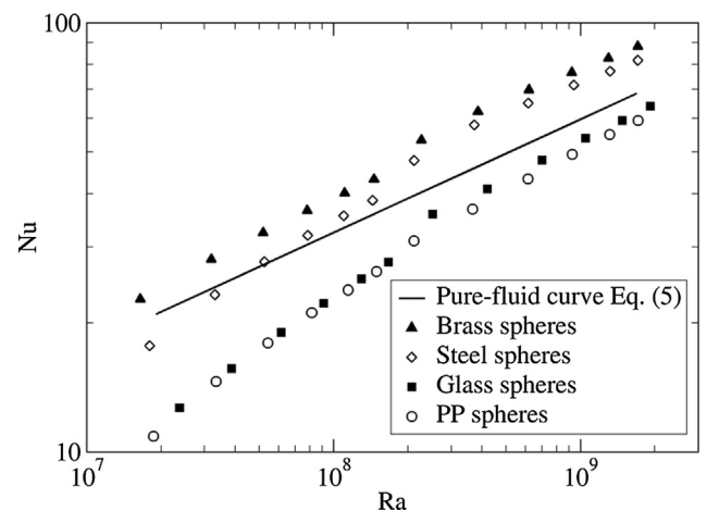
Fig. 6. Effect of sphere conductivity. Nu-Ra data for porous media consisting of 15.3 mm ( d/H = 0.20 ) spheres in BCT packing with different conductivities compared to the pure-fluid reference curve.
