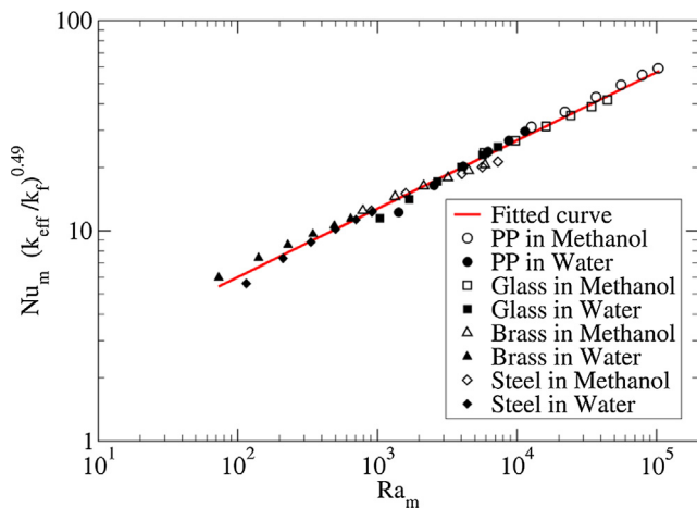
Fig. 8. Heat transfer data based on porous medium dimensionless numbers. Nu_m (k_{eff}/k_f)^{0.49} versus Ra_m for eight different solid-fluid combinations for 15.3 mm ( d/H = 0.20 ) spheres. The red line denotes the fit to the data.
