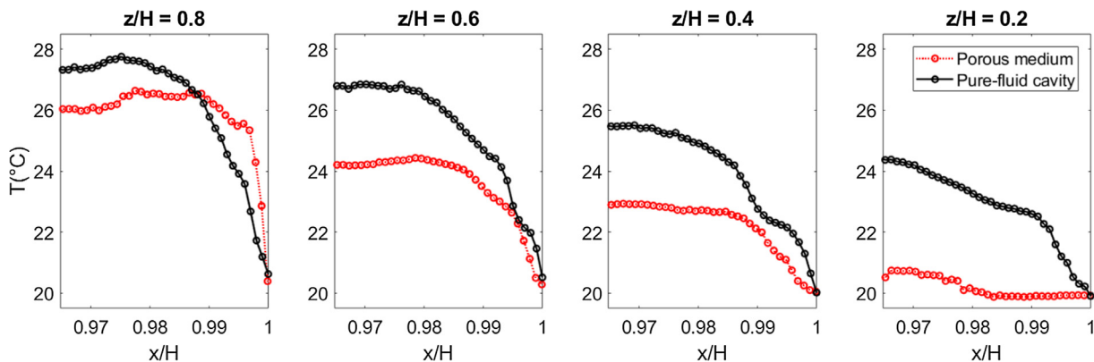
Fig. 18. Temperature profiles along four horizontal lines ( z/H = 0.2, 0.4, 0.6 , and 0.8 ) for the pure-water cavity (black markers), and for the cavity filled with hydrogel spheres (red markers) at Ra = 9.0 \times 10^7 .
