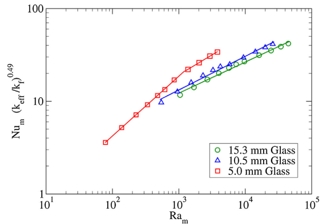
Fig. 9. Heat transfer data based on porous medium dimensionless numbers for three different glass sphere sizes ( d/H = 0.20 , 0.14, and 0.065). The solid lines denote power-law fits to the data.
