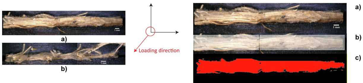
Fig. 9. Cross sectional micrograph with a) horizontally and b) vertically oriented roots with respect to the loading direction.
