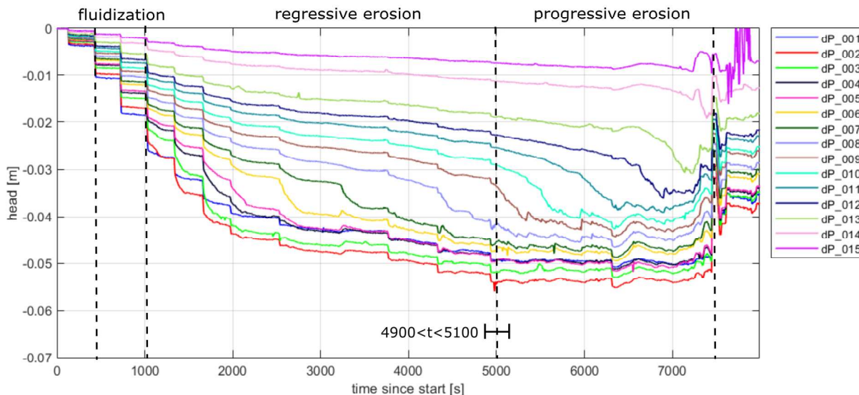
Figure 2. Head development in sensor P1-P15 and erosion phases in test B25_245. “dP” indicates sensors, located from downstream to upstream
