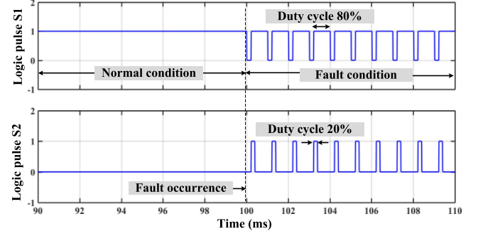
Fig. 12. Control pulse of IGBTs S_1 and S_2 .
