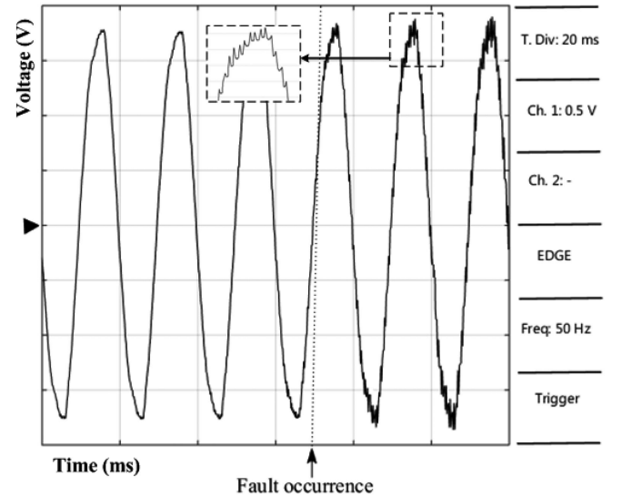
Fig. 15. BESS voltage in normal and fault operation (prob X200).
