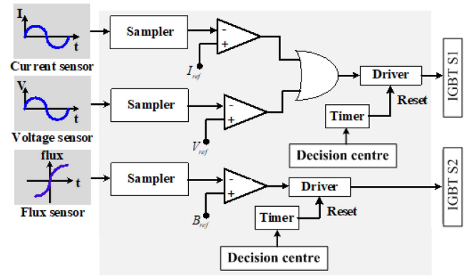
Fig. 6. Controller structure.
