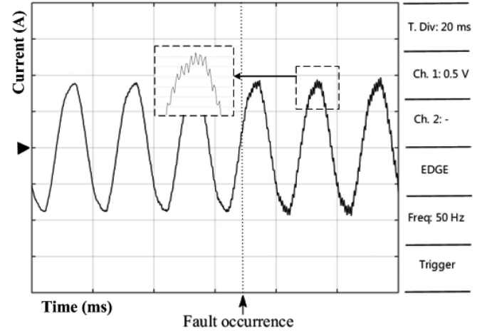
Fig. 14. BESS current in nominal and fault operation (prob X4).
