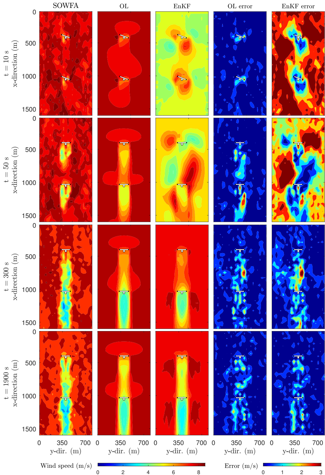
Figure 4: Wind field estimation for t = 10, 50, 300 , and 1900 s. In the left column are the large-eddy simulation (SOWFA) results. The second column shows the open-loop (OL) estimation with grid-searched optimal parameters. The third column shows the estimates using power measurements, initialized with poor values for the wind speed and turbulence. The last two columns show the error between the SOWFA and the OL/EnKF simulation, respectively.
