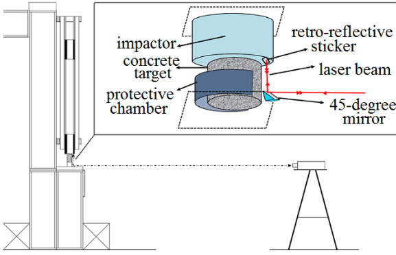
Figure 1: Schematic view of the measurement configuration
