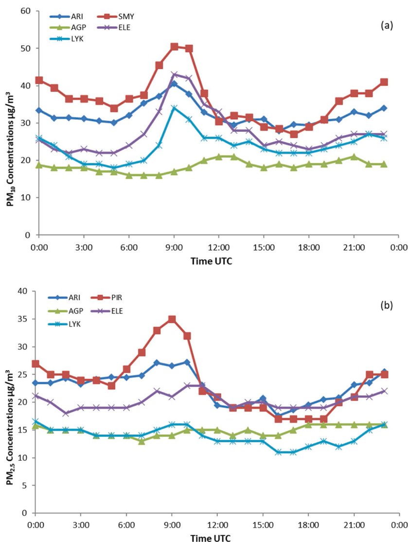
Fig. 5. Hourly average concentrations of local measuring stations: (a) \text{PM}_{10} concentrations (b) \text{PM}_{2.5} concentrations.
