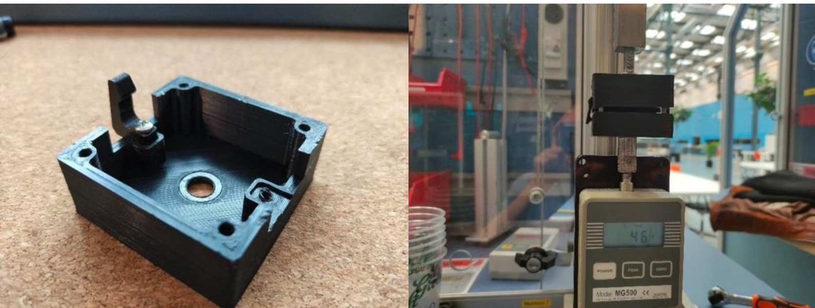
Figure 31 - (left) Jig and (right) force gauge with jig installed to measure tensile and compression forces on snap fits. Used with approval of M. Bakker, 2021.
