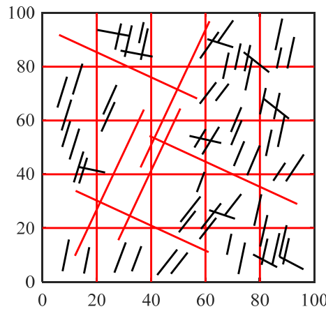
Figure 17 The schematic of a fracture network.
