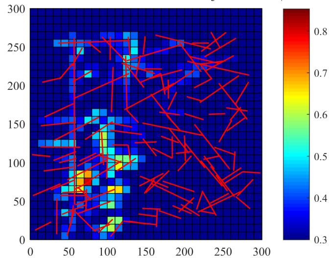
a) The water saturation distribution obtained from DFM (volume weighted)
