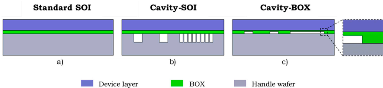
Figure 1. A comparison of three substrate architectures: (a) Standard SOI substrate; (b) Cavity-SOI substrate with cavities in handle wafer; (c) Cavity-BOX substrate with the pre-patterened buried oxide layer.
