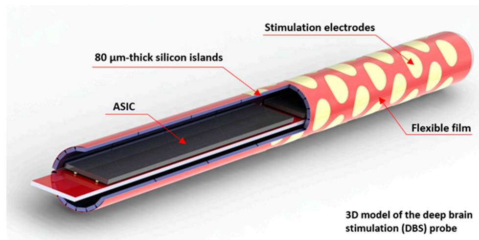
Figure 4. 3D model of the 40-electrode DBS probe ( \varnothing 1.4 mm diameter) with integrated capacitors and ASICs inside the probe's tip.
