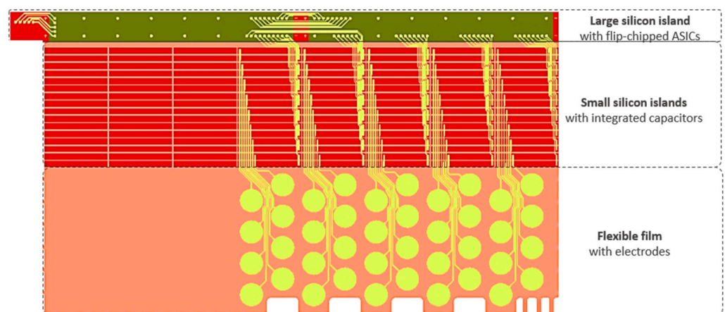
Figure 3. The 2D representation of the 40-electrode DBS design with integrated electronic components. The large silicon island (18 mm \times 1 mm) can contain flip-chipped ASICs. The small silicon islands (210 \mu\text{m} \times 2070 \mu\text{m} ) are separated with 40 \mu\text{m} wide trenches and can accommodate prefabricated decoupling capacitors. The flexible film contains 40 flexible electrodes.
