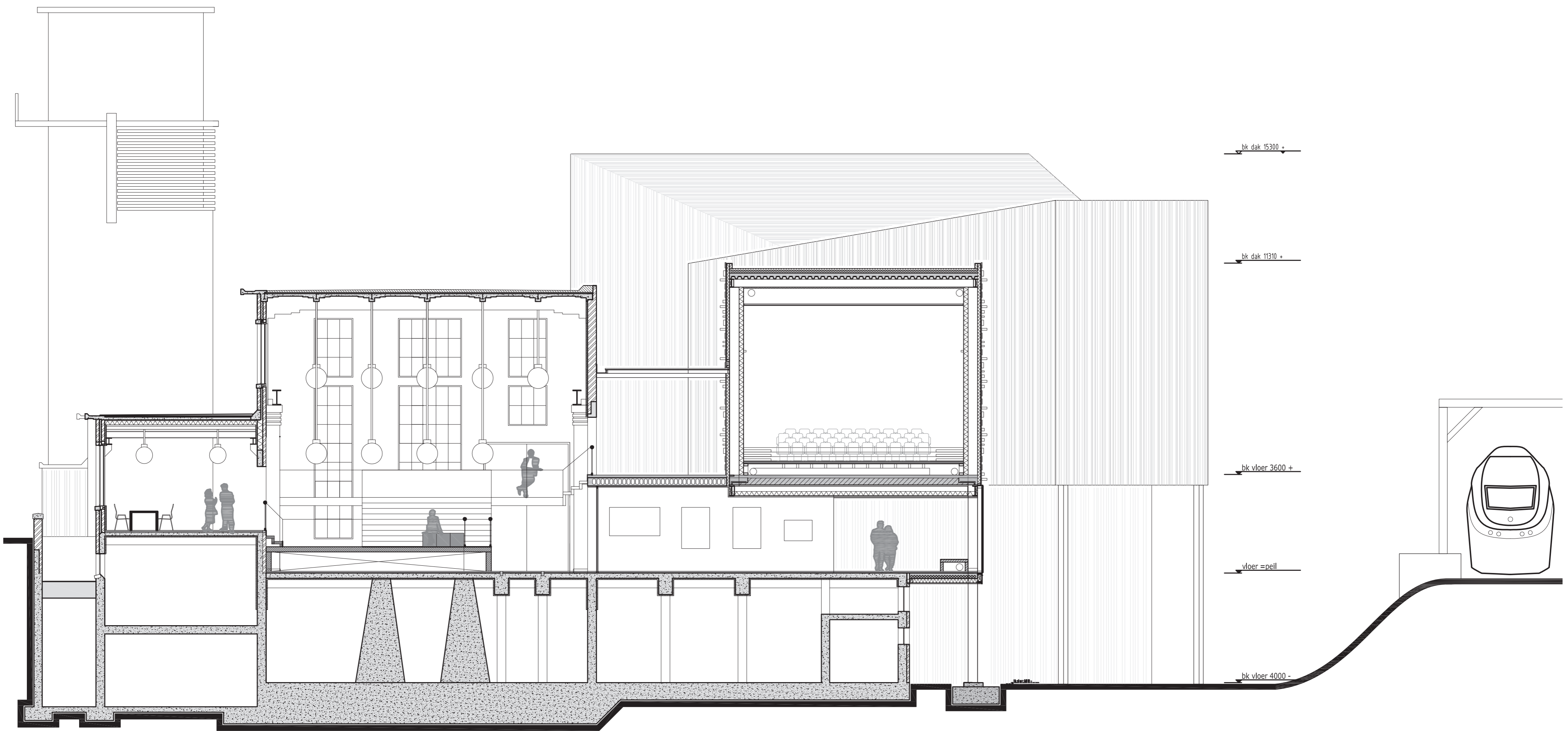
_Dwarsdoorsnede (1:100)
