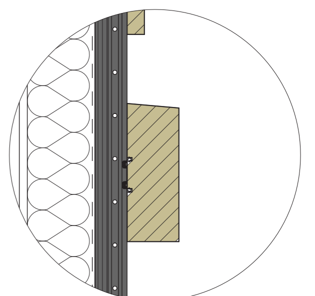
Detail 1 (1:5)
