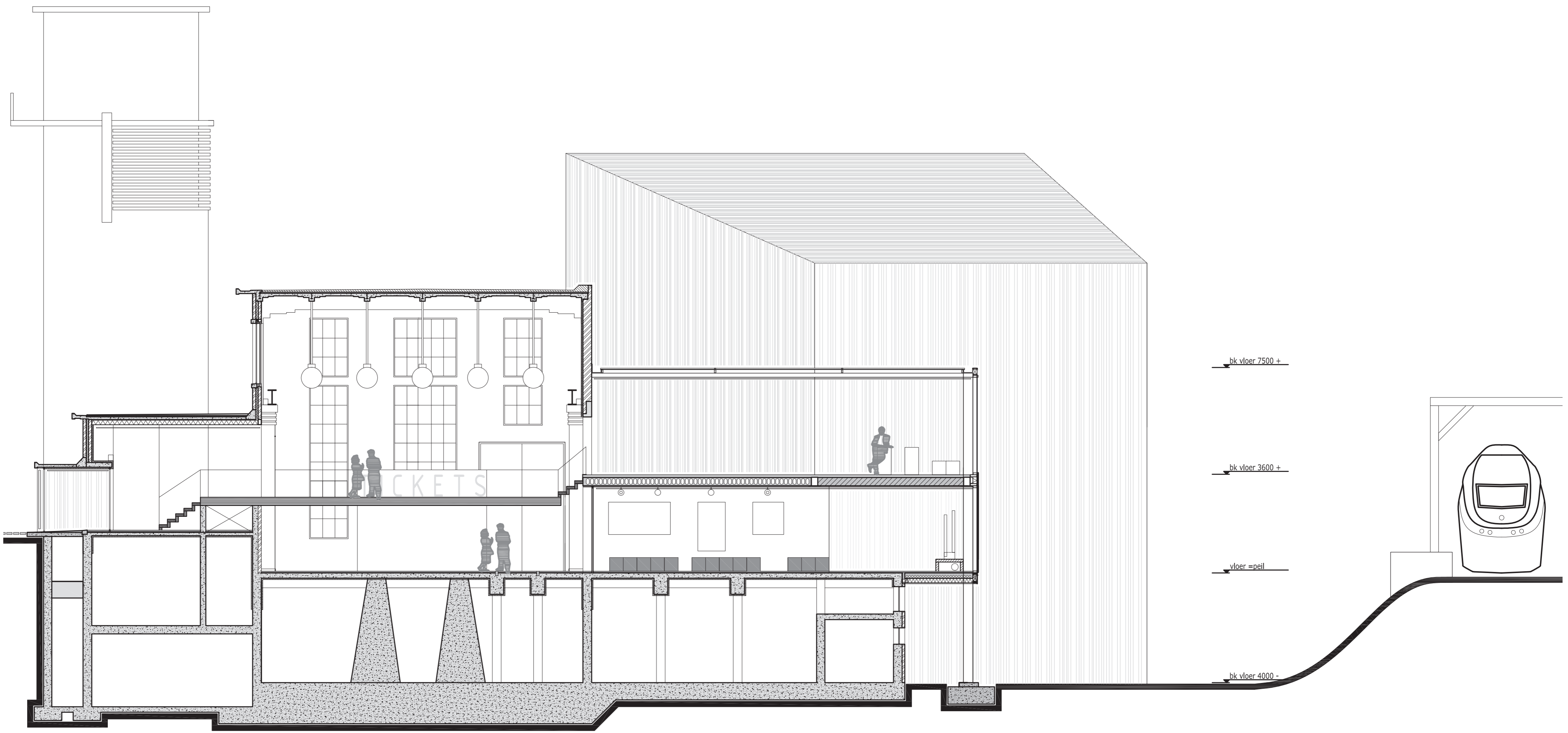
_Dwarsdoorsnede (1:100)
