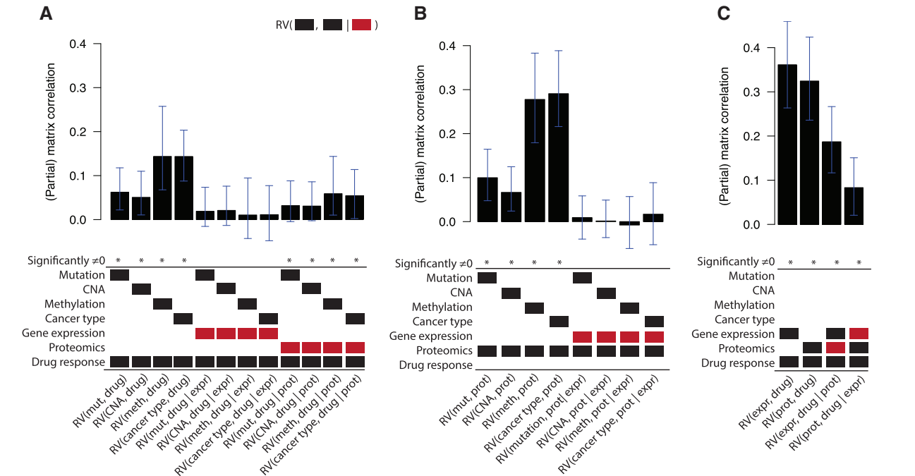
Fig. 6. The (partial) matrix correlations for different RV(X_1, X_2|X_3) in the pharmacogenomics data. For each bar in the barplot, X_1 and X_2 are indicated by the black blocks, and X_3 is indicated by the red block. A (partial) matrix correlation was significant when P < 0.01 . The error bars indicate the 99% confidence interval. mut, mutation; meth, methylation; expr, gene expression; prot, proteomics; drug, drug response
