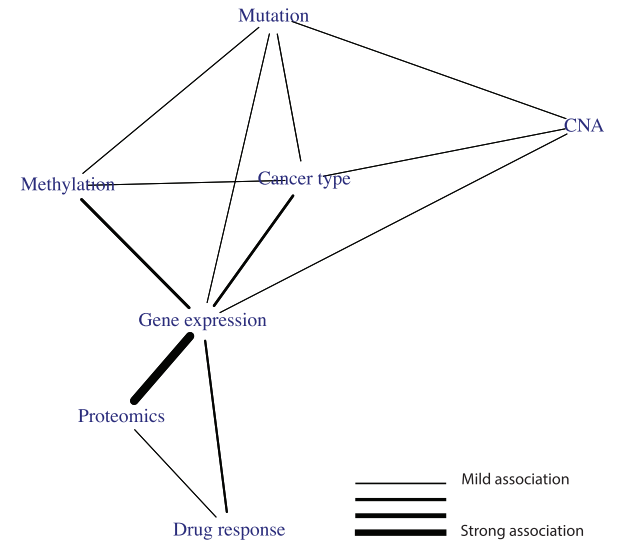
Fig. 5. Relationships between datasets in the pharmacogenomics data, as determined using the PC algorithm run on the partial matrix correlations. An edge indicates that two datasets share information that is not present in any of the other datasets
