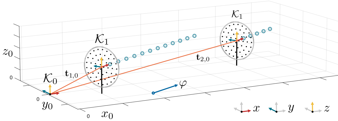
Figure 1. Visualization of the coordinate system \mathcal{K}_0 and the two \mathcal{K}_1 systems of two turbines. The figure also shows the OPs flowing downstream as well as the turbine location vectors \mathbf{t}_{T_i,0} and the wind direction \varphi .
