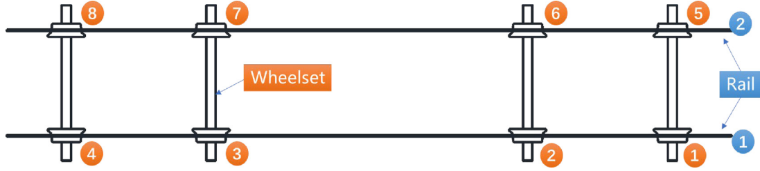
Fig. 3. Schematic drawing of the serial number of primary suspensions.
