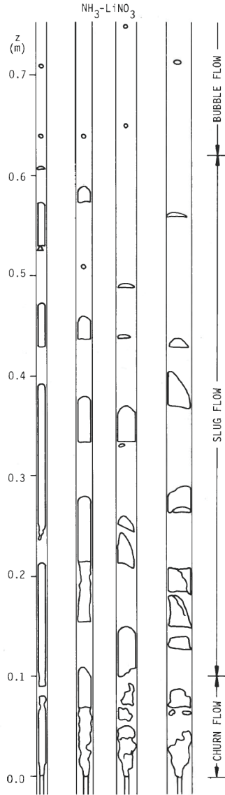
Figure 5.13: Visualizations of flow patterns in \text{NH}_3/\text{LiNO}_3 vertical tubular absorbers with cocurrent upward flows [198]. The ammonia vapor flow is in average 72.5 \times 10^{-6} kg/s, the solution flow 5.5 \times 10^{-3} kg/s.
