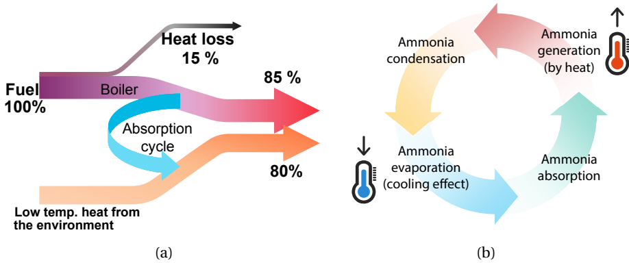
Figure 1.4: Efficient approaches of heating and cooling by using absorption technologies. (a) Heat driven absorption cycles perform better than boilers by reclaiming low temperature heat from the environment; (b) Absorption refrigeration systems achieve cooling effects with a very limited amount of electricity consumption.
