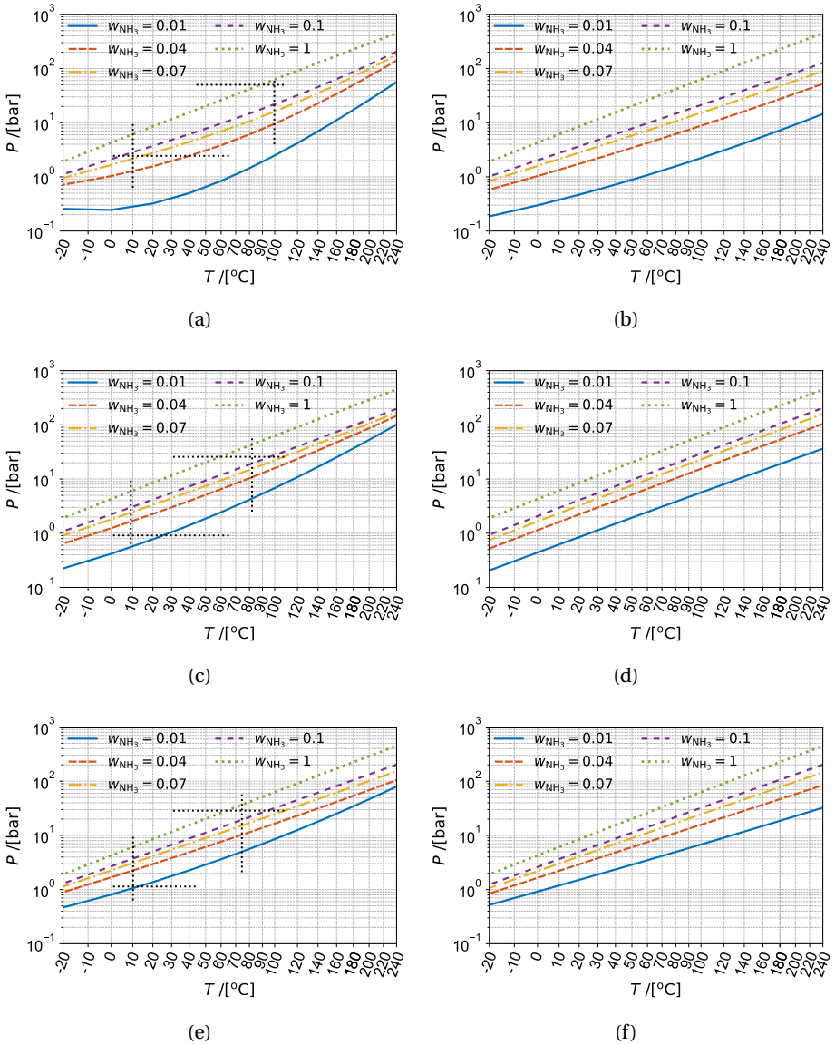
Figure 4.11: Comparison of the vapor pressure curves generated only using the experimental VLE data (EXP) and the ones together using the experimental and simulated VLE data (SIM) for the studied NH 3 /IL working pairs: (a) NH 3 /[emim][SCN] pair (EXP [40]), (b) NH 3 /[emim][SCN] pair (EXP [40] + SIM) (c) NH 3 /[bmim][BF 4 ] pair (EXP [39]), (d) NH 3 /[bmim][BF 4 ] pair (EXP [39] + SIM), (e) NH 3 /[emim][Tf 2 N] pair (EXP [39]), (f) NH 3 /[emim][Tf 2 N] pair (EXP [39] + SIM). Vertical and horizontal dashed lines represent temperature and pressure boundaries of EXP data.
