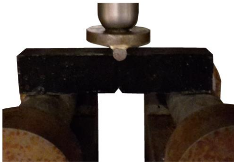
FIGURE 5 (a) Induction heating machine used at laboratory and (b) the three point bending setup with the asphalt mortar specimen used for the induction healing within mould
