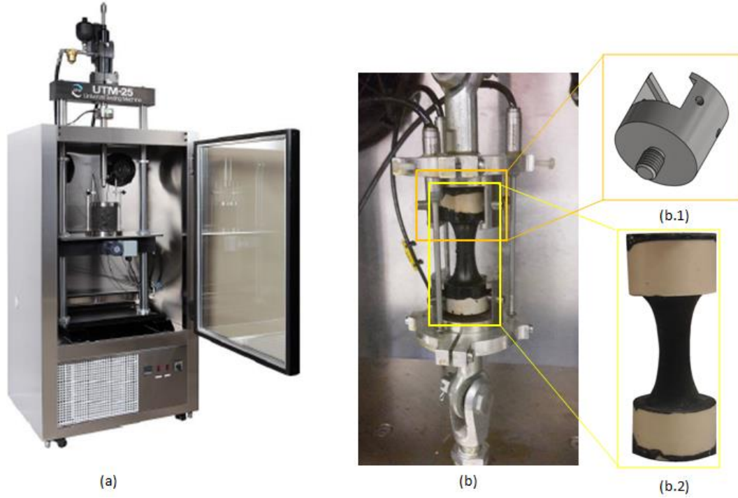
FIGURE 4 Universal Testing Machine UTM-25 (a), the frame (b) with modified hinges (b.1) and asphalt mortar specimen (b.2)
