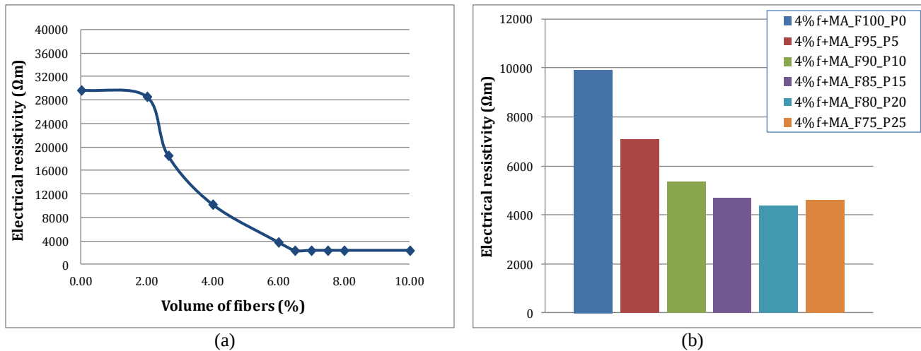
FIGURE 6 Effect of (a) the volume content of steel fibers and of (b) iron powder after substituting mineral filler with iron on the electrical resistivity of asphalt mortars
