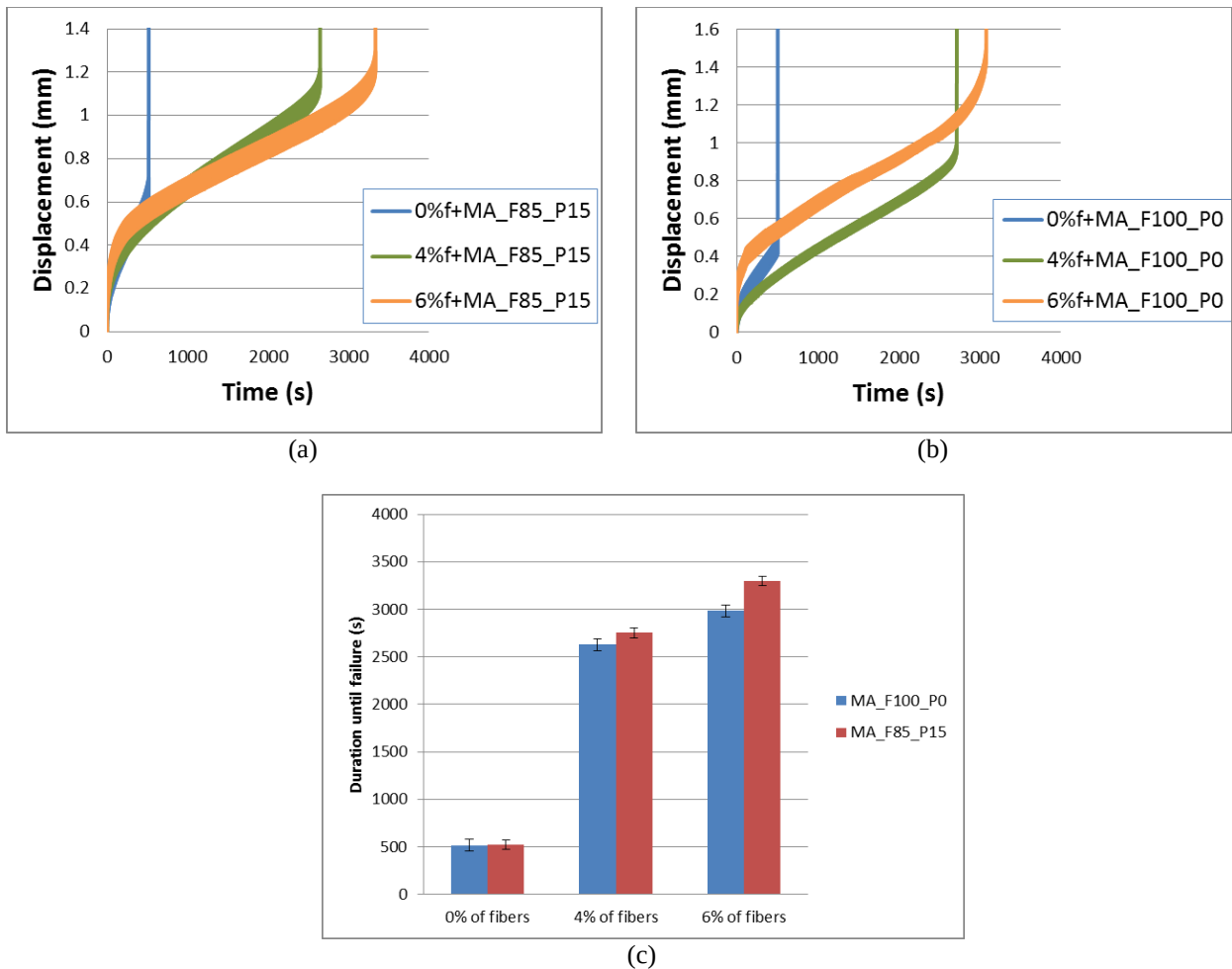
FIGURE 9 Influence of steel fibres on fatigue performance of asphalt mortars (a) with and (b) without iron powder, and (c) the total graph with the fatigue life of different mortars
