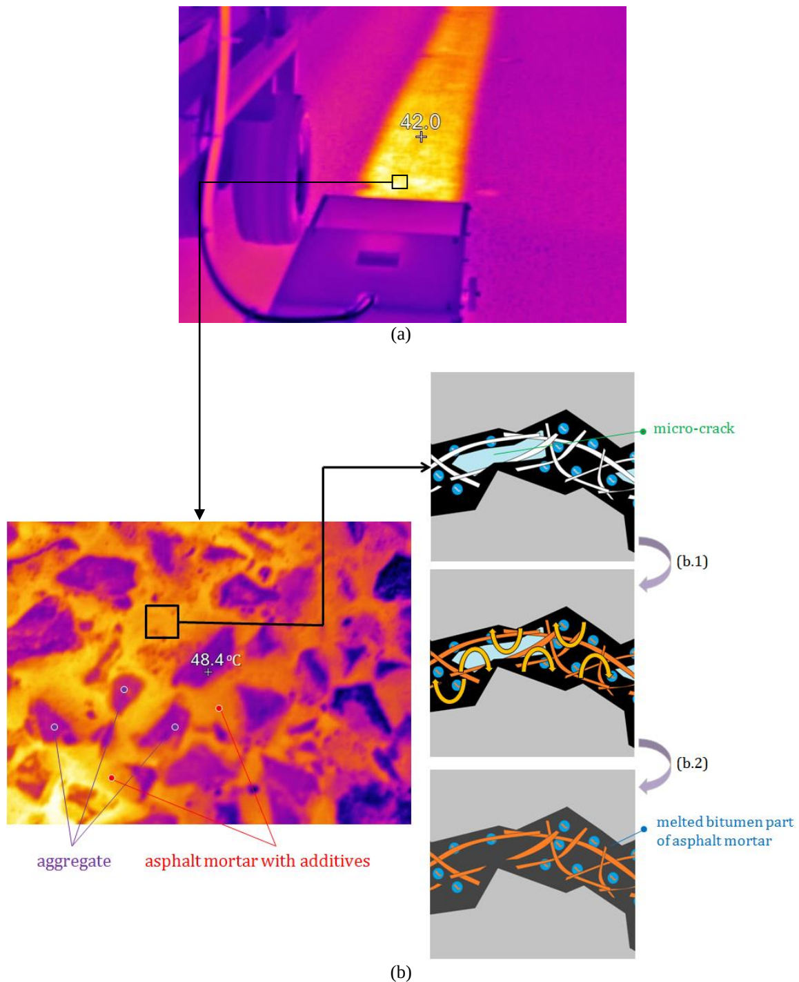
FIGURE 1 Infrared image (a) during induction heating of an asphalt pavement (A58 near Vlissingen, the Netherlands) and (b) of heated asphalt pavement surface at high resolution with the schematic of induction healing, (b.1) asphalt mortar with micro-cracks induced by eddy currents and (b.2) closure of micro-cracks through the heat generation in the asphalt mortar
