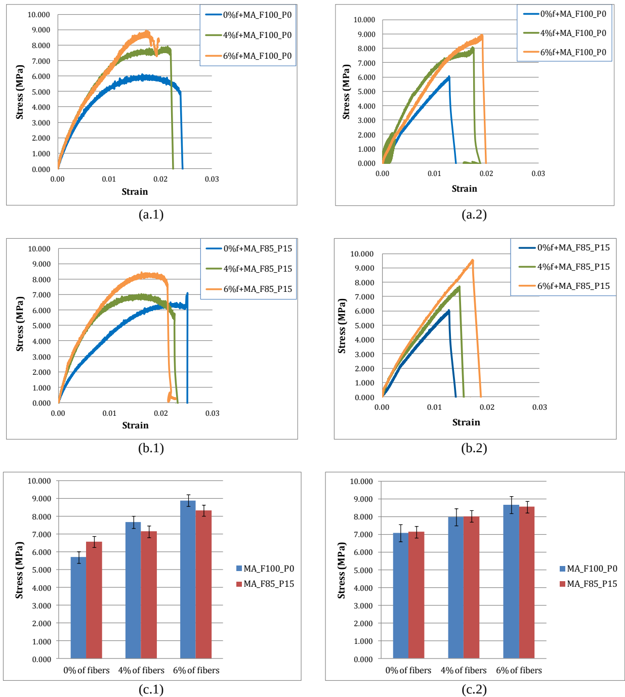
FIGURE 8 Stress-strain curves for asphalt mortars; with mastic MA_F100_P0 and different amounts of fibers, (a.1) displacement rate: 0.0275 mm/s and (a.2) 0.05 mm/s; with mastic MA_F85_P15 and different amounts of fibers, (b.1) displacement rate: 0.0275 mm/s and (b.2) 0.05 mm/s; and the total graphs with the tensile strength of asphalt mortars: displacement rate (c.1) 0.0275 mm/s and (c.2) 0.05 mm/s
