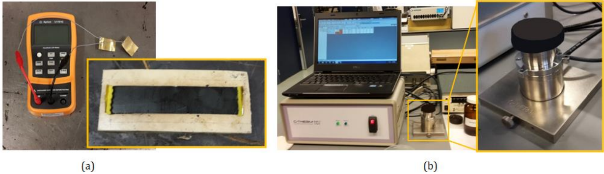
FIGURE 3 (a) Digital multimeter for electrical resistivity measurement and (b) C-Therm TCi thermal analyzer for thermal properties measurements
