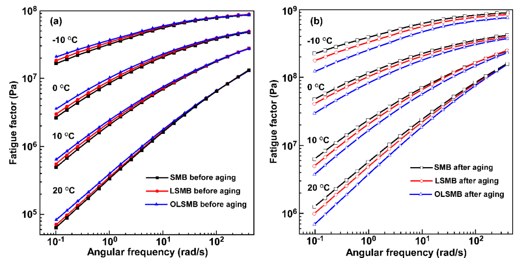
Figure 7. Fatigue factor vs. frequency for SMB, LSMB and OLSMB (a) before and (b) after aging.
