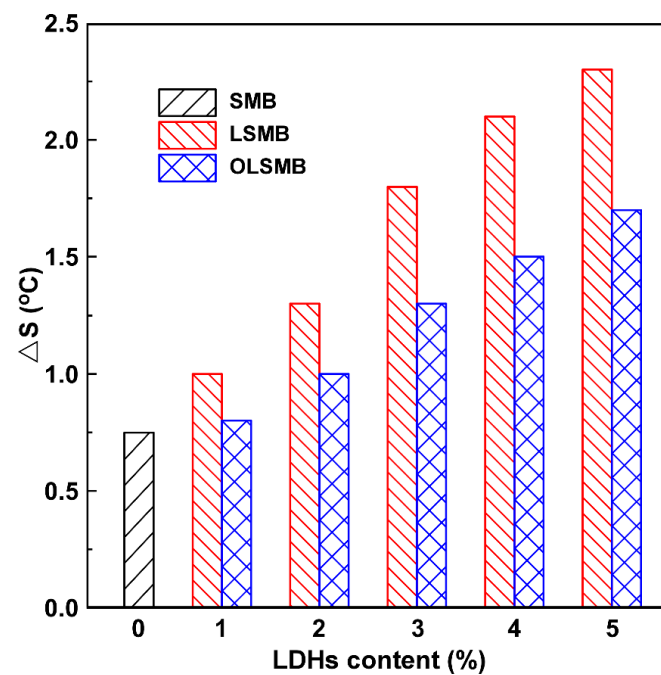
Figure 2. The storage stability of SMB, LSMB and OLSMB.
