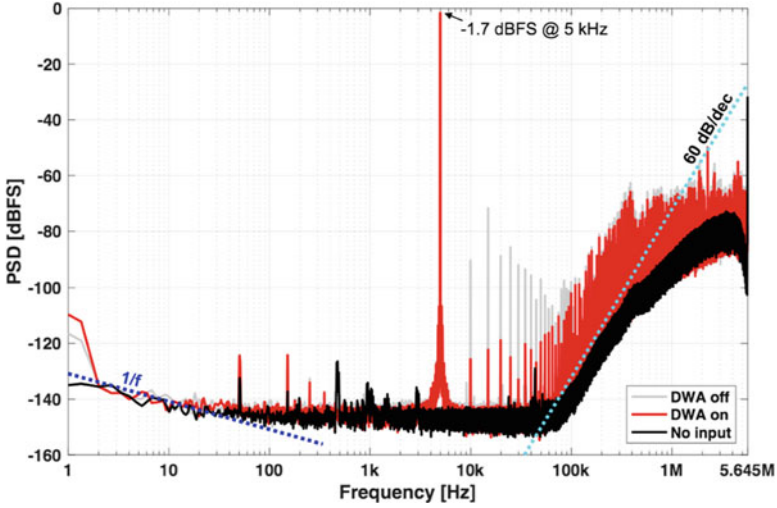
Fig. 6.16 Measured output spectra for DWA off, DWA on, and no input. Inputs are connected to V_{CM} for no input case, with DWA on
