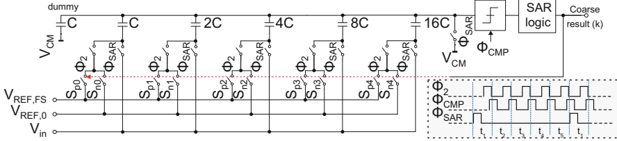
Fig. 6.14 The SAR ADC
