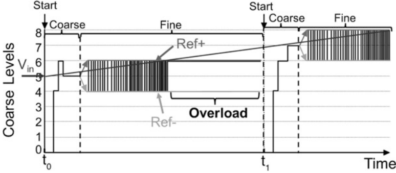
Fig. 6.6 Time-domain operation of an incremental zoom ADC with a dynamic input. Showing the SAR ADC's comparator output during the coarse period, and the SDM's bitstream during the fine period
