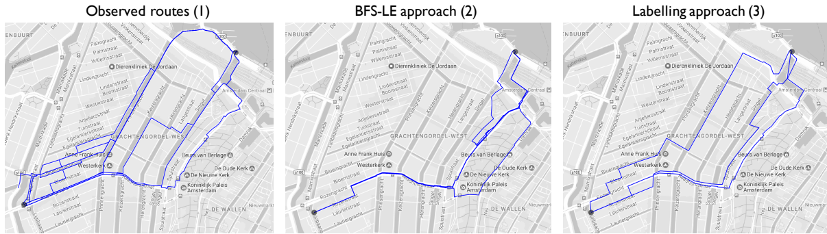
Figure 6.5: Routes generated for a given OD pair from the West of Amsterdam to the central train station, for (1) observed routes, (2) BFS-LE approach and (3) Labelling approach.
