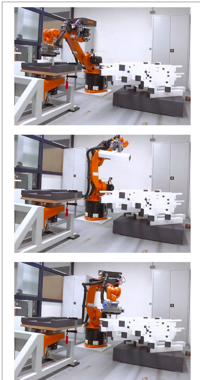
FIGURE 4 | Working path for stacking involved movement sequences such as picking, transporting, and placing.
