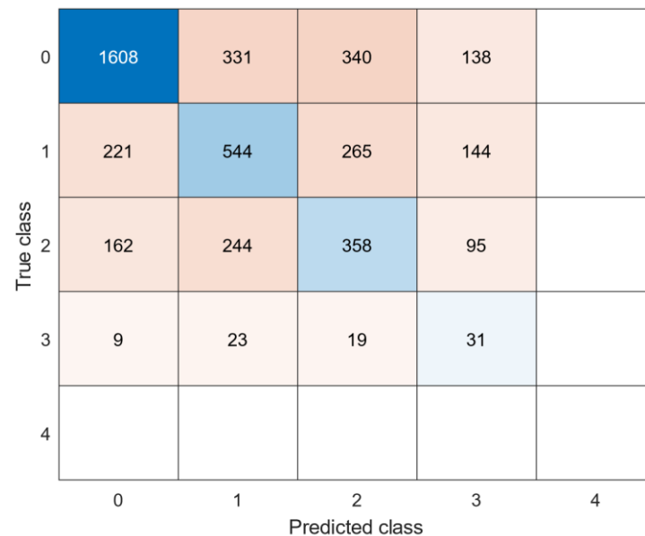
Figure 4. Confusion matrix: generalized model of lower extremities dystonia.
