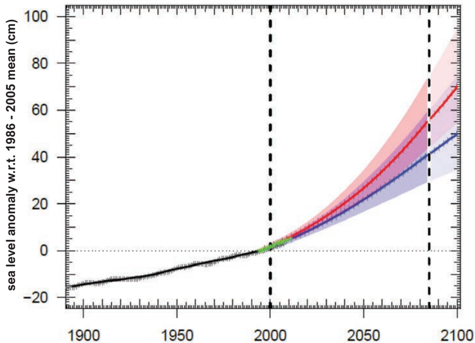
Figure 2.10: Eustatic sea level rise projections based on the KNMI '14 scenarios (modified from KNMI, 2014).
