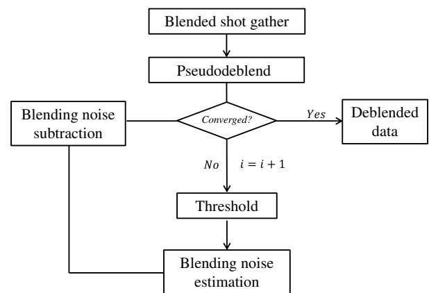
Figure 4. The workflow of the deblending method in the case of shot repetition.
