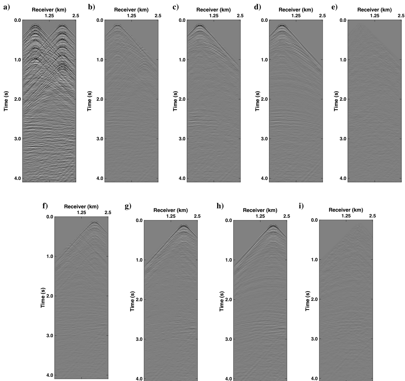
Figure 5. Field-data example: (a) numerically blended shot gather, (b) pseudodeblended shot gather A, (c) debblended shot gather A, (d) original shot gather A, (e) the debblending error of shot gather A (c-d), (f) pseudodeblended shot gather B, (g) debblended shot gather B, (h) original shot gather B, and (i) the debblending error of shot gather B (g-h).
