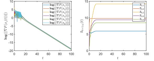
Fig. 2. Global gradient \nabla F(\cdot) evaluated at x_i(t) (in a logarithmic scale), i \in \mathcal{V} (left). Adaptive coupling gains \bar{a}_{k+1,i_k}(t) , k \in \mathcal{I}_5 , in \bar{\mathcal{G}}^* (right). Here, \gamma_1 = \gamma_2 = 0.5 .
