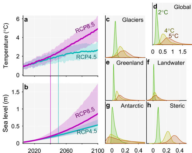
Fig. 1. Projections (5%, 50%, and 95% quantiles) of (A) global average surface temperature and (B) global sea level rise since 2005, with dates when expected global mean temperature rises 2 °C. (C–H) The sea level pdfs for the individual components, and for combined global sea level rise for warmings of 2 (green), 4 (yellow) and 5 °C (brown): (C) glaciers, (D) global, (E) Greenland, (F) land water, (G) Antarctic, and (H) steric. The x axis is sea level (meters) and y axis is probability density.
