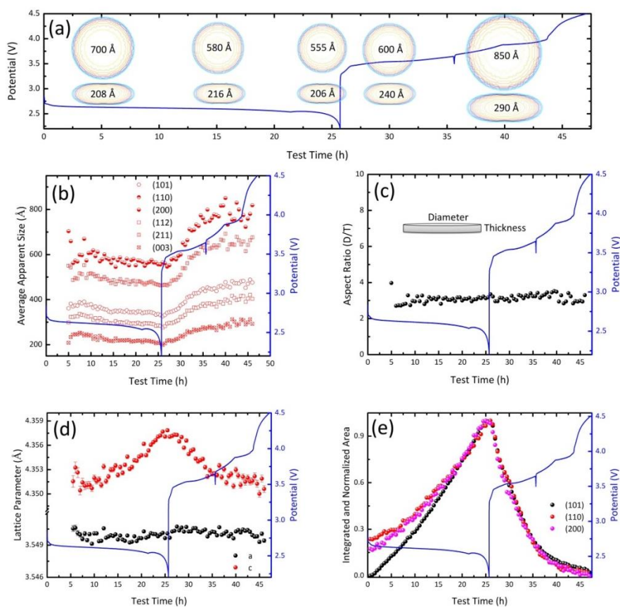
Figure S2.11. (a) The evolution of the LiOH crystallite shape, (b) the evolution the average apparent size, (c) the aspect ratio of the LiOH crystallite shape (diameter in the ab-plane/thickness in the c-direction), and (d) LiOH lattice parameters, resulting from Rietveld refinement as a function of time during the full galvanostatic (dis)charge cycle. (e) The evolution of the integrated and normalized area as a function of discharge time for {101}, {110} and {200} reflections of LiOH. The battery test was performed in a DME/LiI based electrolyte with moist \text{O}_2 at a current density of 0.3 \text{ mA/cm}^2 .
