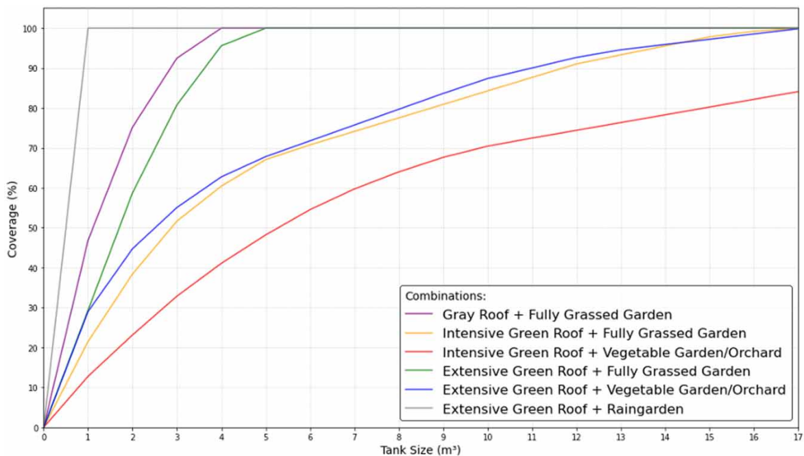
Figure 5 | BGI combinations efficiency: additional external water demand coverage (%) by tank size (m 3 ).
