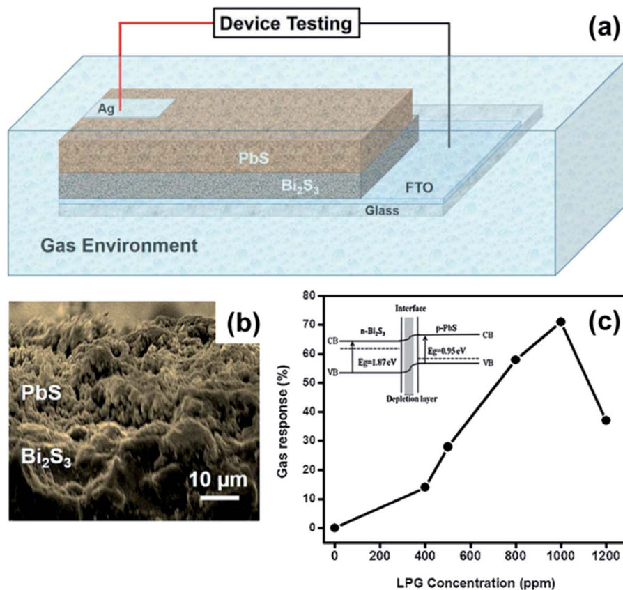
Fig. 23 (a) Schematic representation of the n- \text{Bi}_2\text{S}_3 /p- \text{PbS} heterojunction device. (b) SEM image of the n- \text{Bi}_2\text{S}_3 /p- \text{PbS} heterojunction. (c) The plot of variation in gas response (%) vs. LPG concentration (ppm) of the n- \text{Bi}_2\text{S}_3 /p- \text{PbS} heterojunction. The inset shows the band diagram of the n- \text{Bi}_2\text{S}_3 /p- \text{PbS} heterojunction. Reprinted with permission from ref. 177. Copyright 2017, Elsevier.
