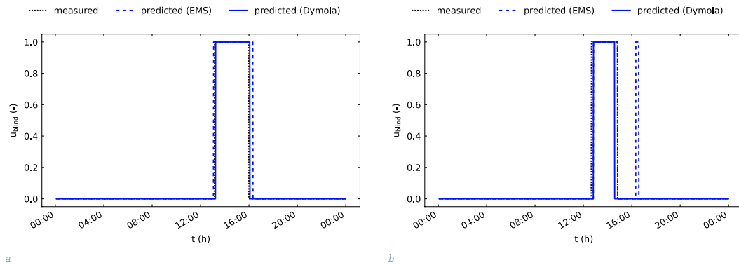
FIG. 17 Comparison of measured and predicted blind positions (0: blinds open, 1: blinds closed) for two representative days.
