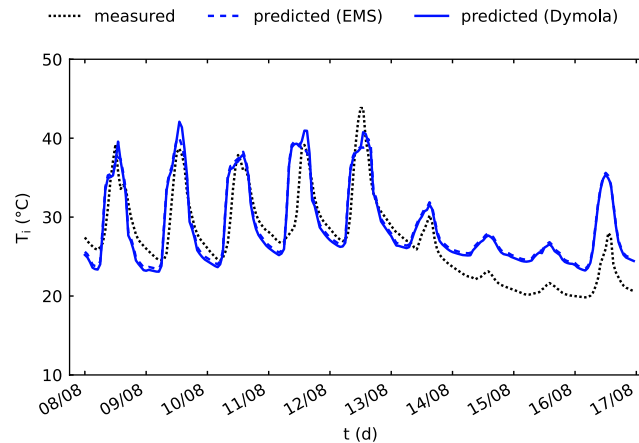
FIG. 16 Comparison of measured and predicted T_i in the validation of the co-simulation model.
