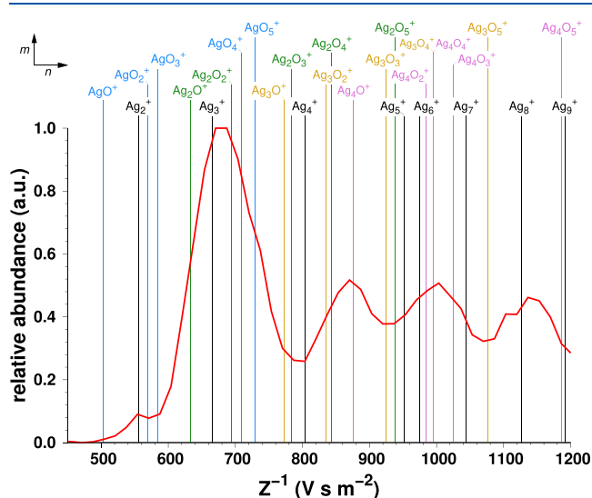
Figure 6. Inverse electrical mobility, Z^{-1} , (in \text{V s m}^{-2} ) of \text{Ag}_n\text{O}_m^+ clusters ( n = 1-4 ; m = 1-5 ) and \text{Ag}_n^+ clusters ( n = 2-9 ) in He calculated at 20^\circ\text{C} and 1 atm. Z^{-1} values of \text{Ag}_n\text{O}_m^+ clusters have been calculated by the trajectory method (TM), and for \text{Ag}_n^+ , the clusters are based on the experimental collision cross sections reported in the literature (ref 17). They are both labeled as vertical lines on the experimental mobility spectrum provided by Maisser et al. (solid red lines, ref 13).
