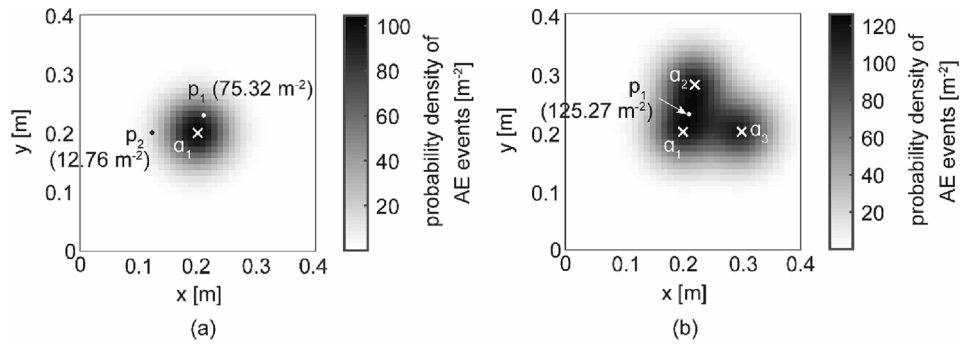
Fig. 2. Illustration of probability density field of (a) one AE event and (b) multiple AE events.
