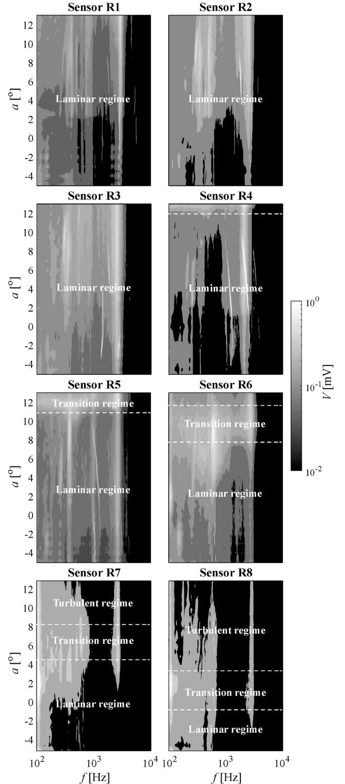
Fig. 7. Measured voltage, V , of segment 2 as a function of frequency, f , and angle of attack, \alpha , without morphing the wing ( \delta = 0 mm).
