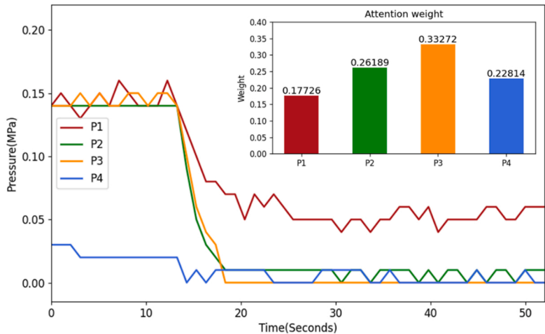
b) Pressure variation by sensors at various positions, i.e., P1, P2, P3, and P4, and the predicted weight value of each sensor
