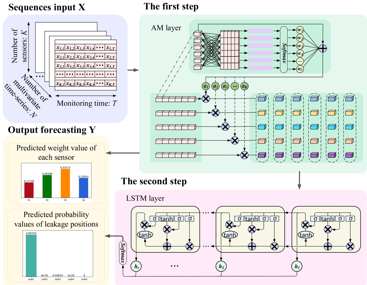
Fig. 1. Architecture of the proposed AM-LSTM approach.
