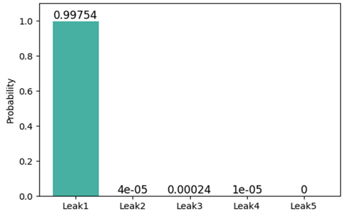
a) Predicted probability values of various leakage positions, namely leak1, leak2, leak3, leak4, leak5
