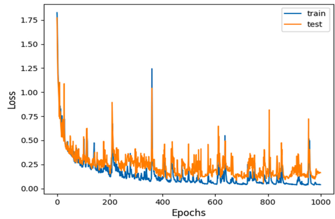
Fig. 4. Loss curves for 1000 epochs generated by AM-LSTM training and testing.
