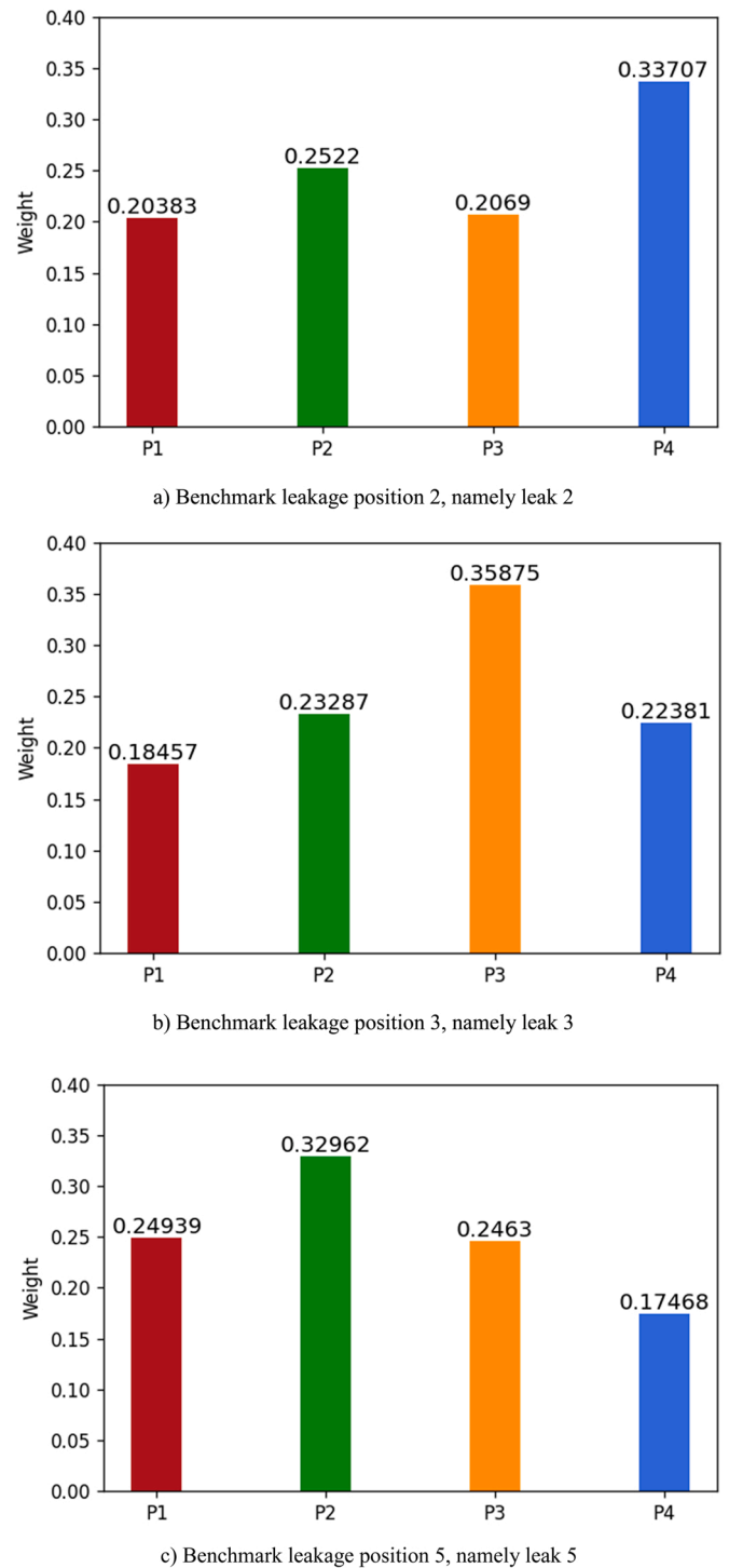
Fig. 11. Attention weights to 4 sensors, namely P1 to P4, under the same benchmark leakage conditions as in Table 2.
