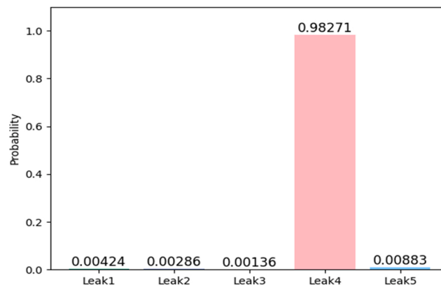
a) Predicted probability values of various leakage positions, namely leak 1, leak 2, leak 3, leak 4, leak 5
