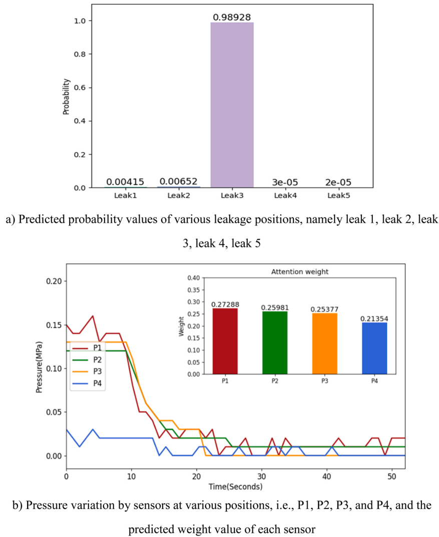
Fig. 7. Real-time automated leakage detection results under operation pressure 0.15 MPa and leak 3.
