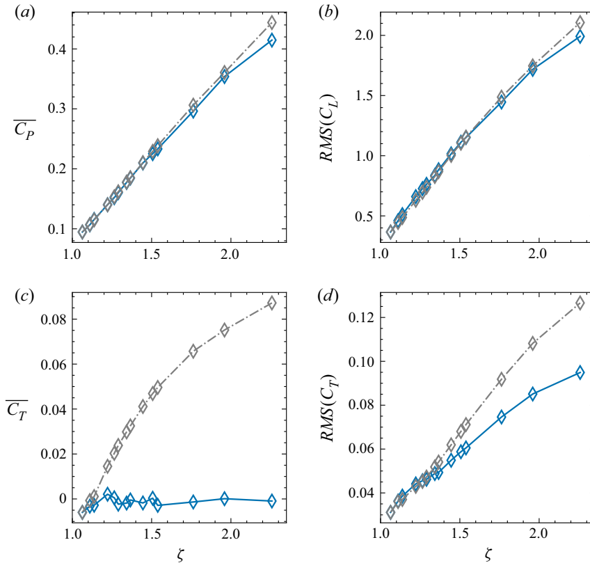
Figure 8. The key swimming performance and force characteristics of the plate at Re = 12\,000 . (a) The power required to maintain SPS. (b) The side force RMS. (c) The time-averaged thrust. (d) The RMS thrust. The points making up the solid line are the rough simulations, and the dash-dotted line is a kinematically equivalent smooth simulation that matches \zeta to the rough case.
