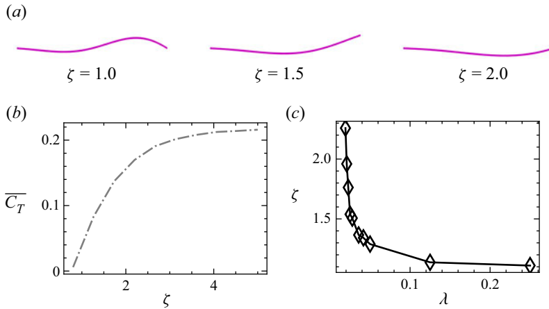
Figure 3. The impact of \zeta on (a) the shape of and (b) the forces on a smooth plate. (c) The required wave speed \zeta for SPS of a rough plate, given different wavelengths ( \lambda ).
