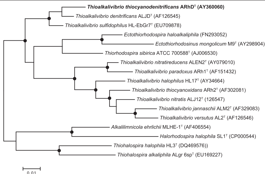
Fig. 1 16S rRNA phylogenetic tree of the described Thioalkalivibrio species, as well as various organisms belonging to the family of Ectothiorhodospiraceae . Nodes with a bootstrap value between 90–100 % are marked with black dots. The outgroup, members of the Alphaproteobacteria , are pruned from the tree. The tree was constructed in ARB [15] and the bootstrap values calculated using MEGA6 [16]
