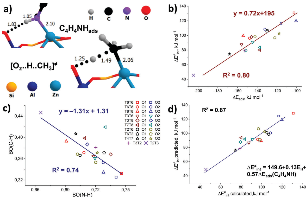
Fig. 6 The use of pyrrole as a multifunctional adsorption probe for the reactivity of Zn_{EF}^{2+} \cdots O_F^{2-} Lewis acid-base pairs. A comparison of the transition state for C-H cleavage and pyrrole adsorption complex geometries for the T8T8O1 configuration (a). Correlations between the intrinsic activation barrier and pyrrole adsorption energies (b). Correlation between bond orders of C-H and N-H in transition states and pyrrole adsorption complexes (c). Two-dimensional correlations between \Delta E_{int}^\ddagger and a linear combination of \Delta E_{ads}(CH_3CN) and E_H (d). " \Delta E_{int}^\ddagger predicted" is the activation energy value predicted using the linear combination of \Delta E_{ads}(C_4H_4NH) and E_H , while " \Delta E_{int}^\ddagger calculated" refers to the DFT-calculated activation energy.
