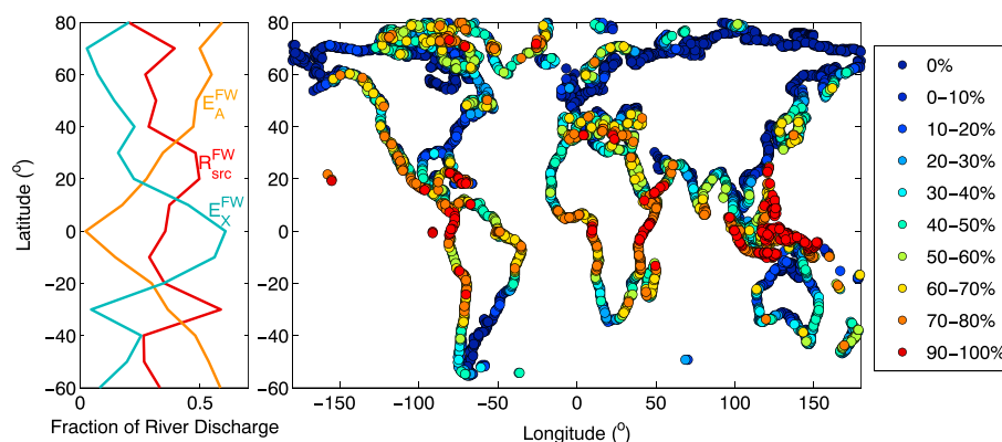
Figure 4. Estimated global freshwater export. (a) Cross-shelf and alongshore export ( E_X and E_A ) and near source retention ( R_{src} ) of riverine fresh water in 10^\circ latitude bands. (b) Cross-shelf freshwater export efficiency beyond the 200 m isobaths for individual rivers in the GlobalNews model.
