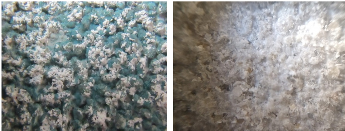
Fig. 8. Left: Dendritic salt efflorescence on panel A1, 3 months after the application; Right: salt crust on the surface of panel A2, 6 months after the application (right).
