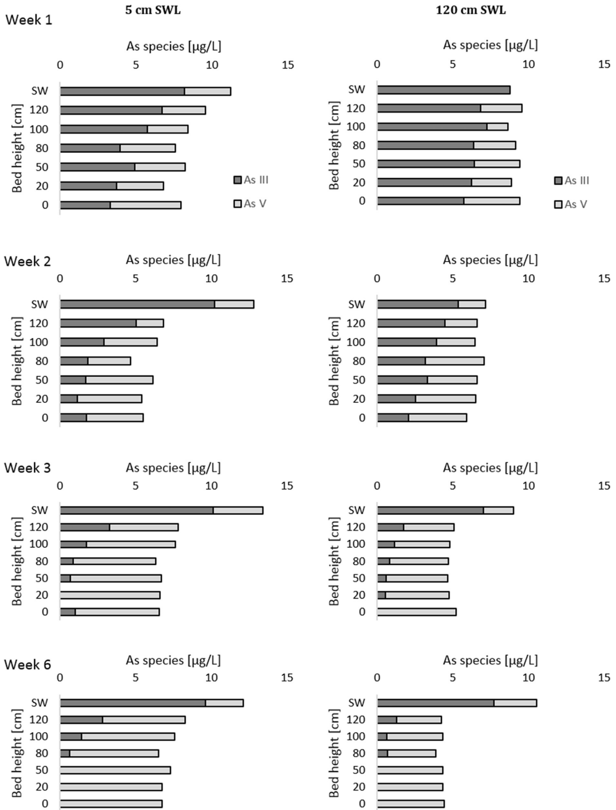
Fig. 3. As(III) and As(V) speciation of dissolved As over the filter bed height for 5 cm SWL (left) and 120 cm SWL (right) with filtration velocity of 1.5 [m/h] for day 1, 8, 15, 36.
